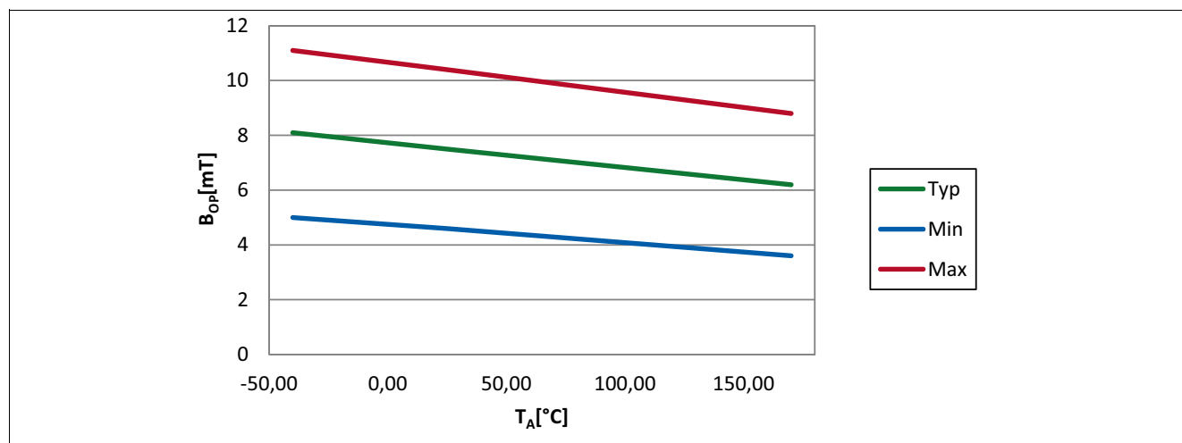
Figure 16 Operating point ( B_{OP} ) of the TLE4961-3K over temperature
