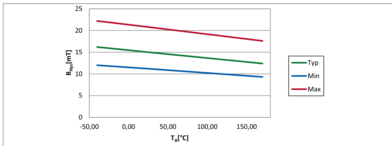
Figure 18 Hysteresis ( B_{Hys} ) of the TLE4961-3K over temperature
