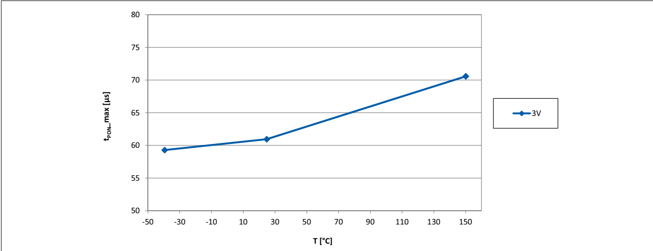
Figure 19 Power on time t_{PON} of the TLE4961-3K over temperature
