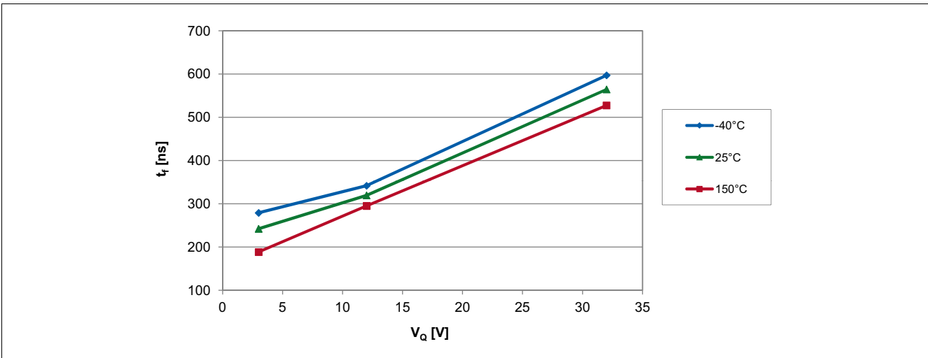
Figure 26 Output fall time of the TLE4961-3K over applied pull-up voltage
