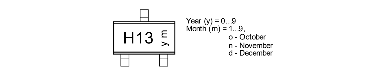
Figure 15 Marking of TLE4961-3K
