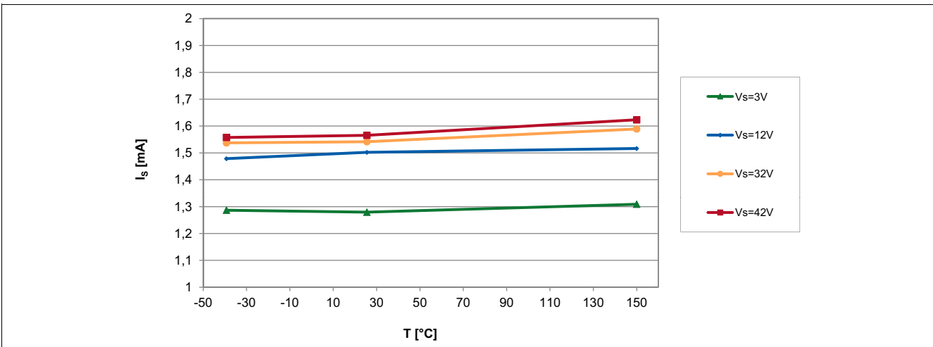
Figure 21 Supply current of the TLE4961-3K over temperature
