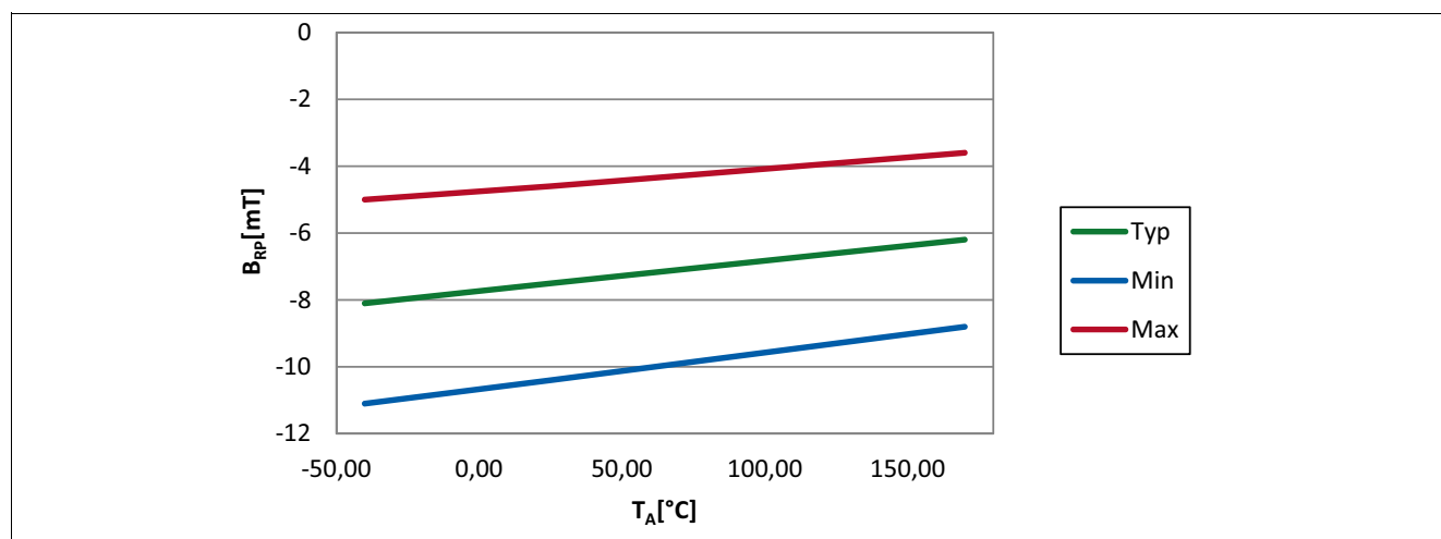
Figure 17 Release point ( B_{RP} ) of the TLE4961-3K over temperature
