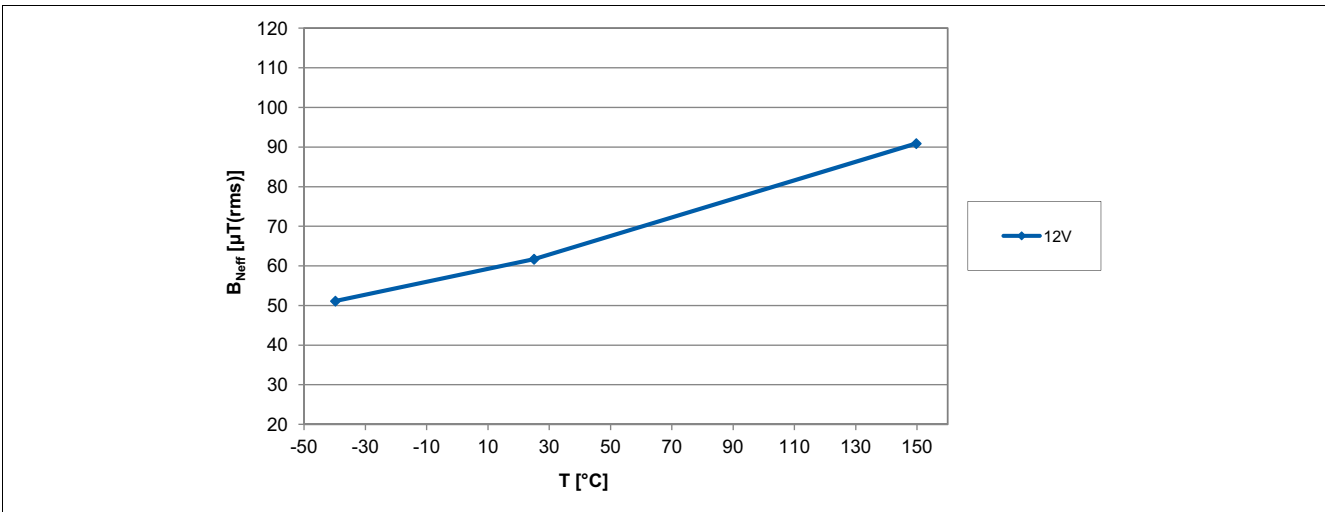
Figure 32 Effective noise of the TLE4961-3K thresholds over temperature
