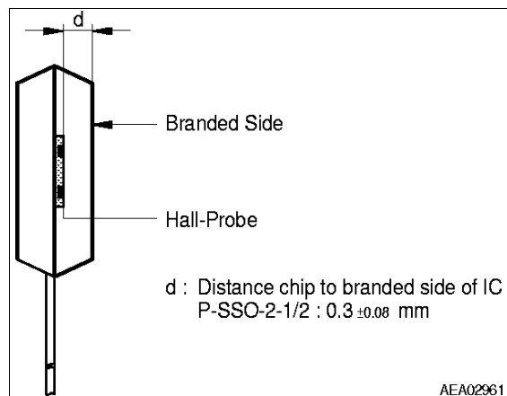
Figure 4-2 Package Outline
