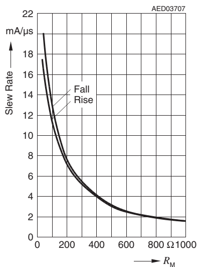
Slew Rate with C = 1.8 \text{ nF} = f(R_M)
