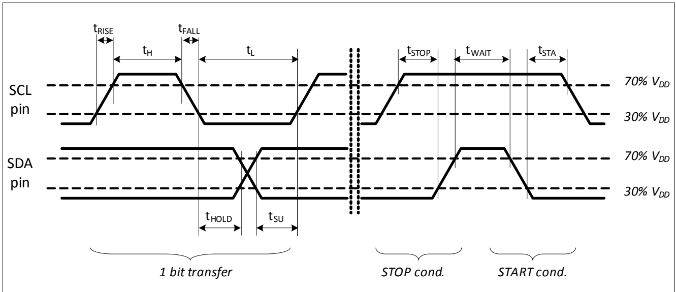
Figure 8 I²C timing specification
