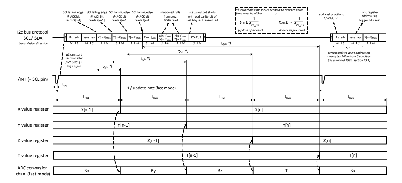
Figure 7 I²C readout frame, ADC conversion and related timing
