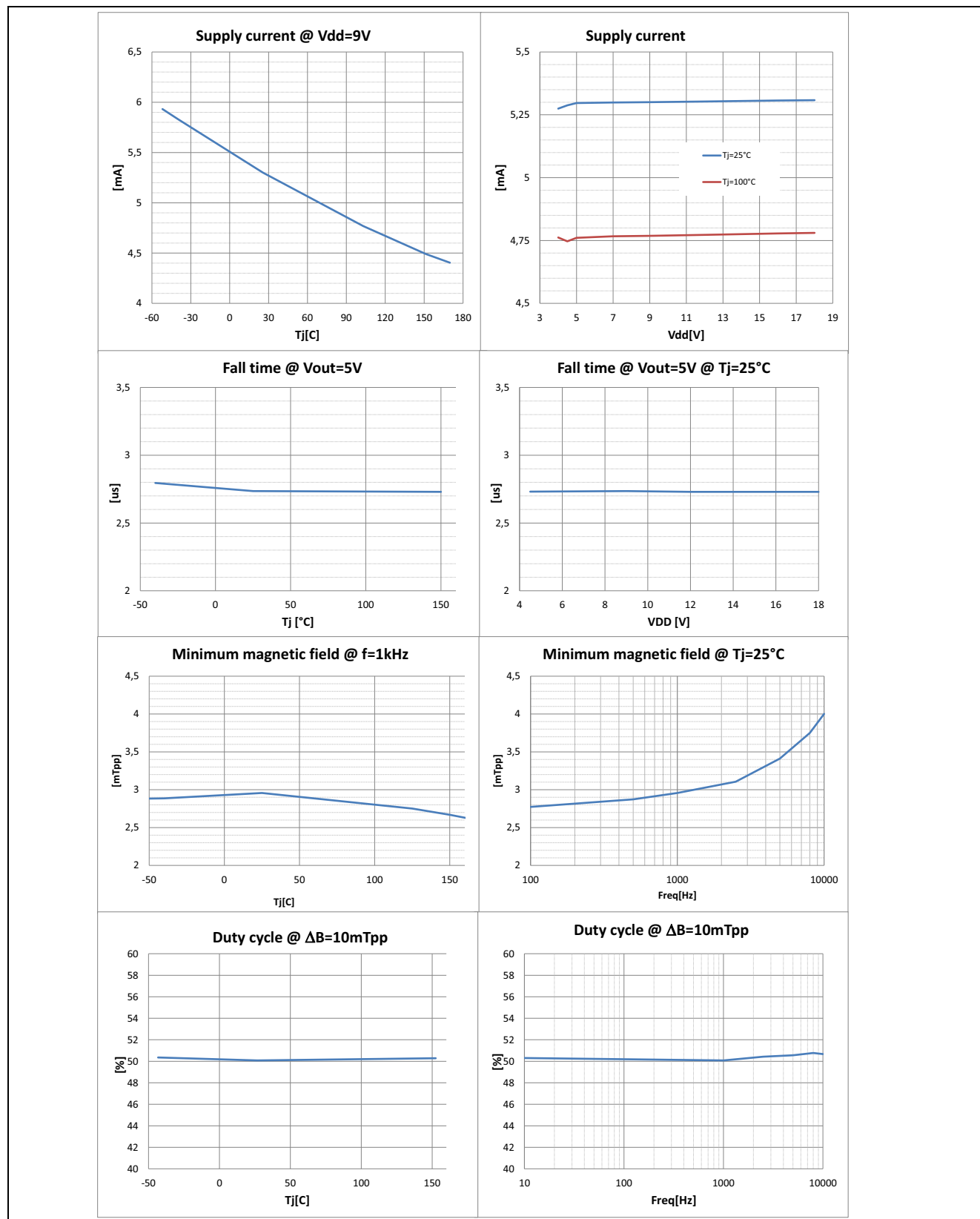
Figure 2-3 Typical Performance
