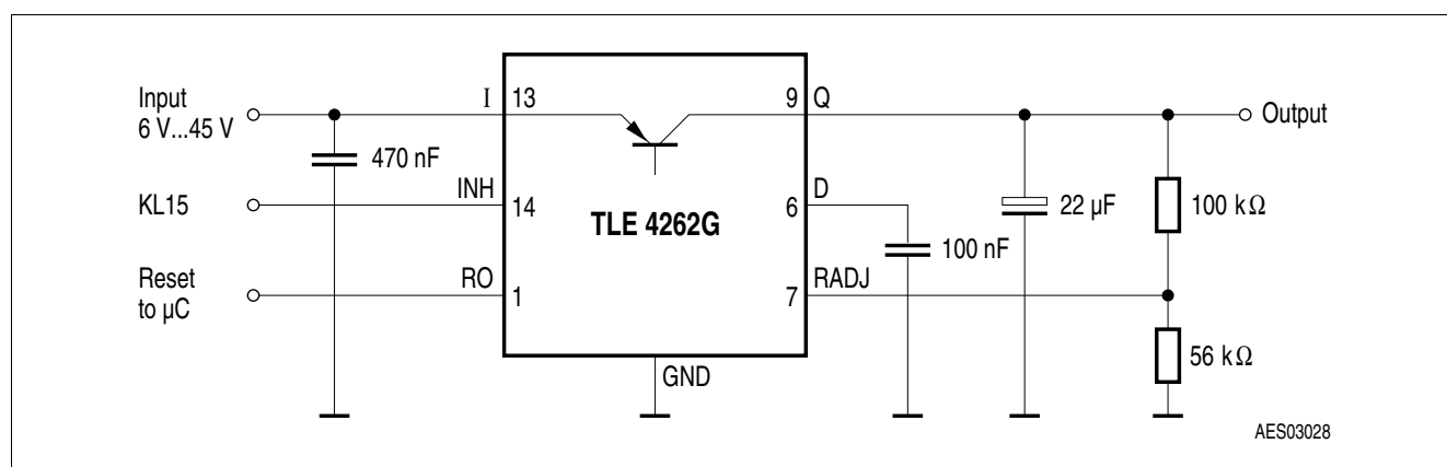
Figure 3 Application circuit
