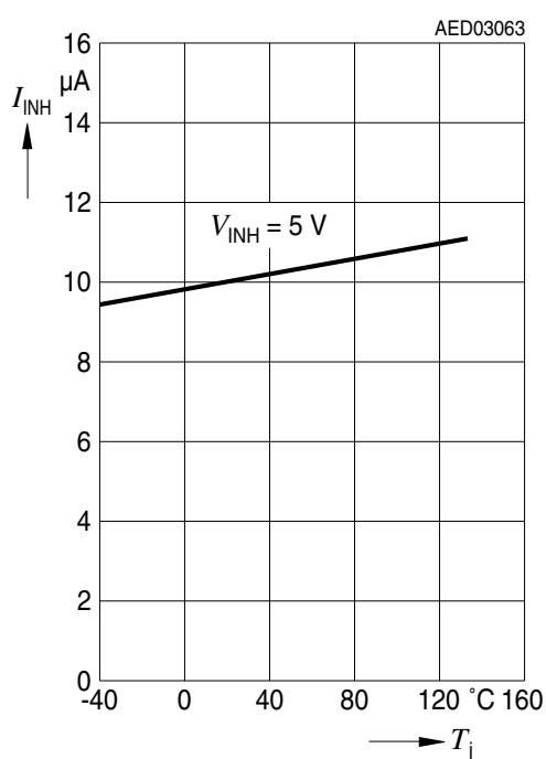
Current consumption of inhibit I_{INH} versus junction temperature T_j
