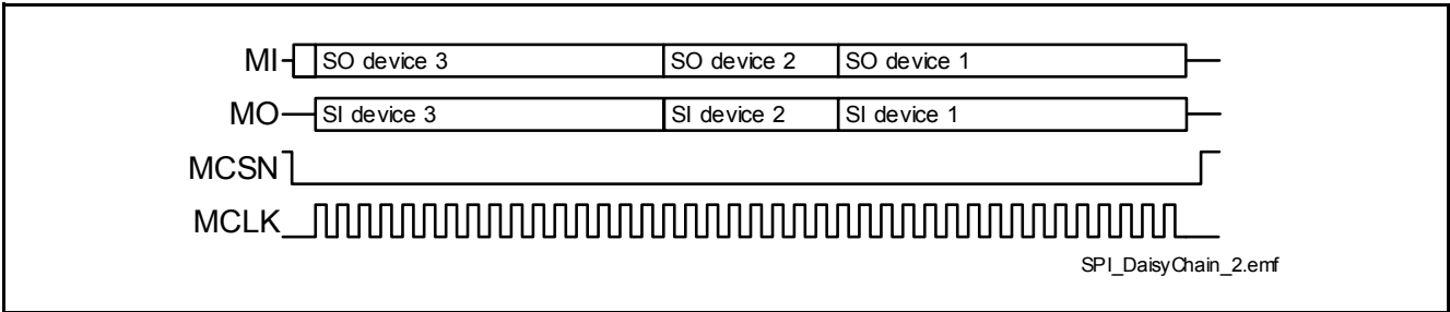
Figure 30 Data Transfer in Daisy Chain Configuration
