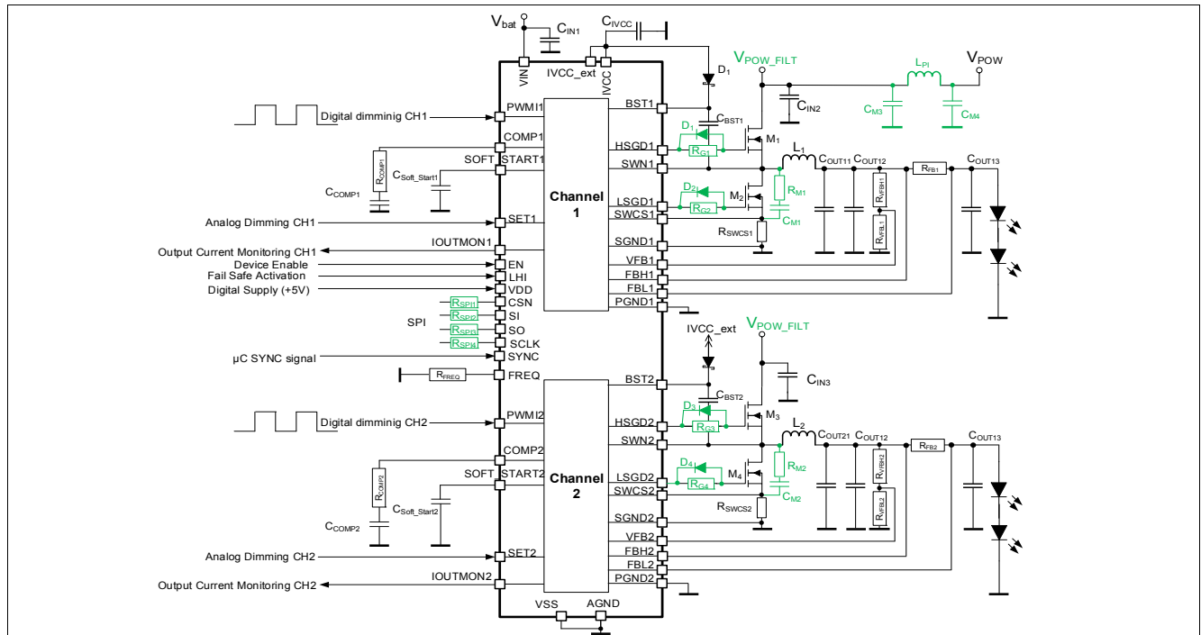
Figure 26 Application Drawing Including Additional Components for an Improved EMC Behavior - TLD5501-2QV
