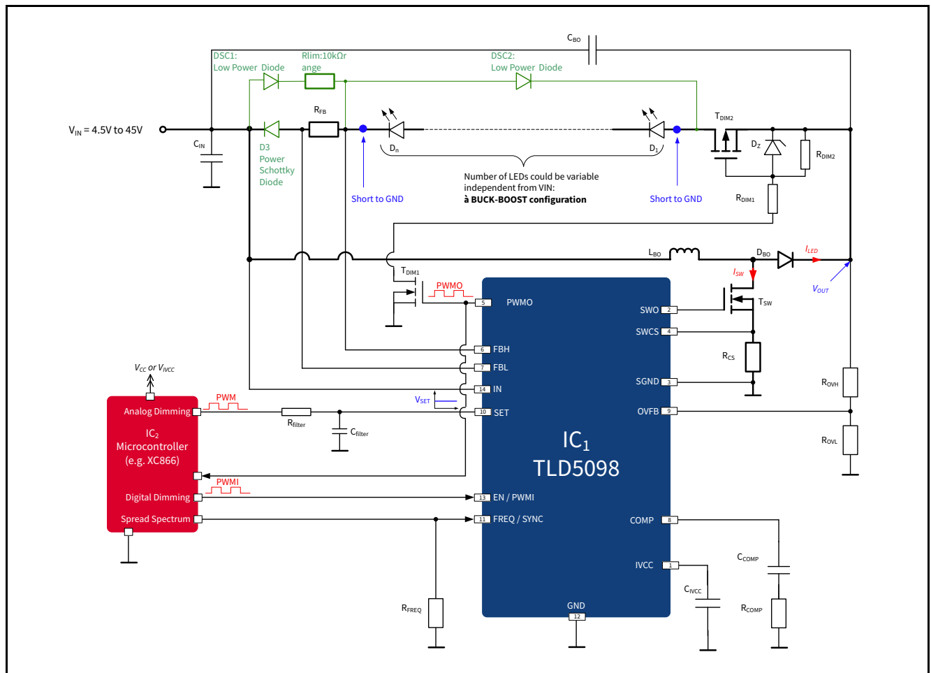
Figure 26 Boost to Battery application circuit - B2B (Buck - Boost configuration)
