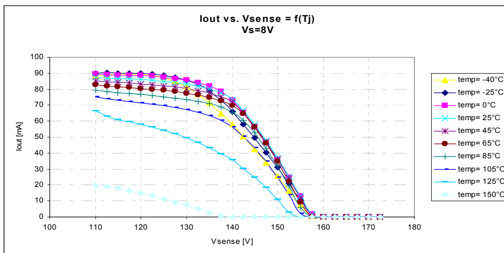
Figure 9 I_{out} vs V_{sense} = f(T_j) at V_s = 8\text{ V}
