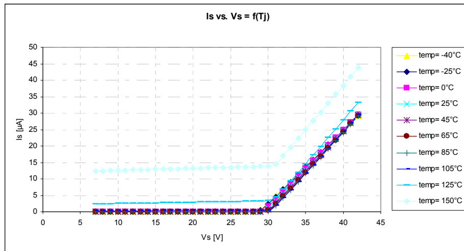
Figure 15 I_s vs V_s = f(T_J)
