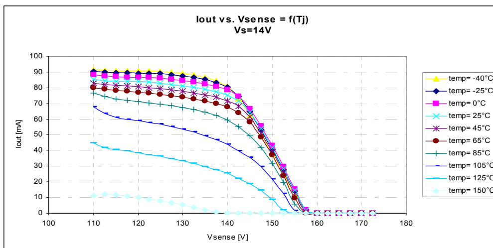
Figure 10 I_{out} vs V_{sense} = f(T_j) at V_s = 14\text{ V}
