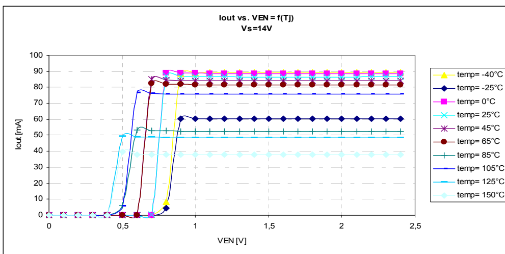
Figure 12 I_{out} vs V_{EN} = f(T_J) at V_s = 14\text{ V}
