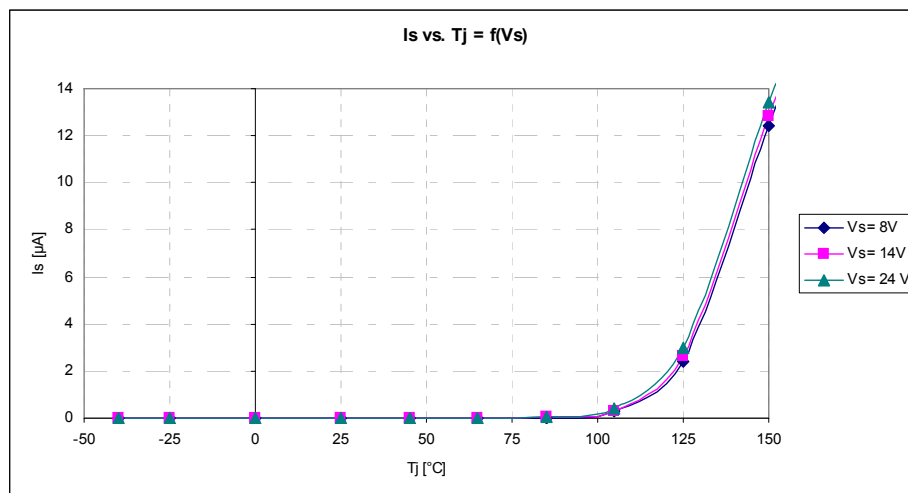
Figure 13 I_s vs T_j = f(V_s)
