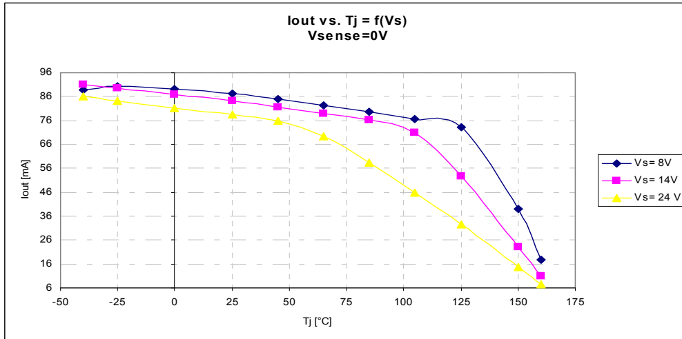
Figure 7 I_{out} vs T_J = f(V_s)
