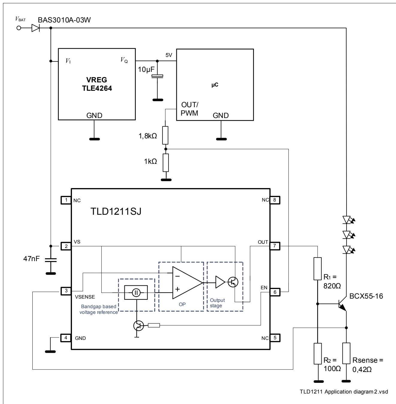
Figure 16 Application Information with External Output Stage
