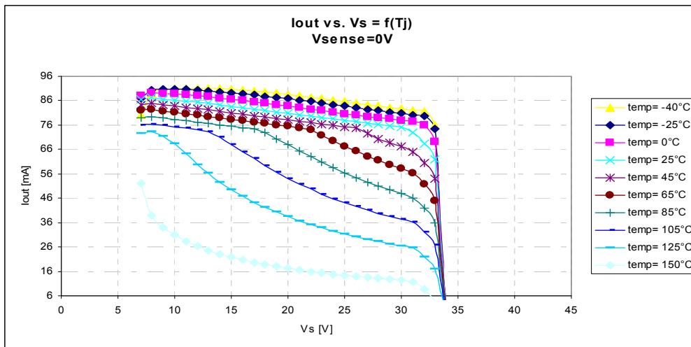
Figure 8 I_{out} vs V_s = f(T_J)
