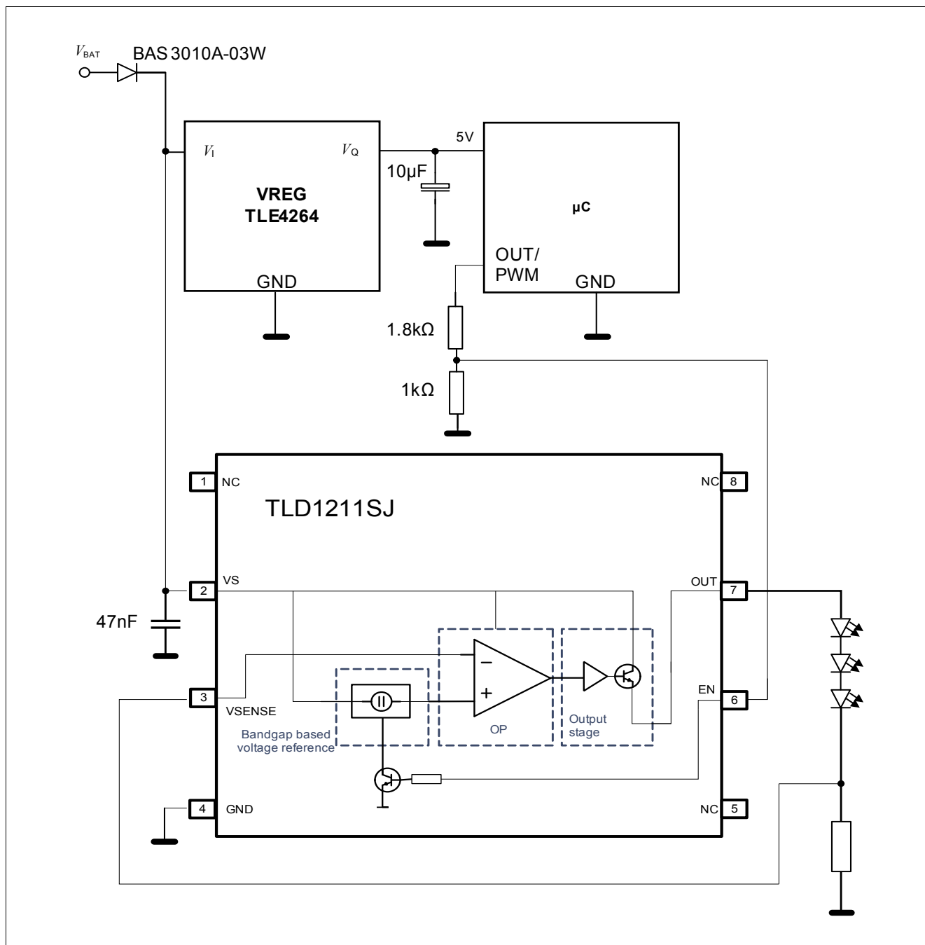
Figure 17 Application Information with Integrated Output Stage Usage
