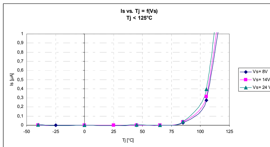
Figure 14 I_s vs T_j = f(V_s) , T_j < 125^\circ\text{C}
