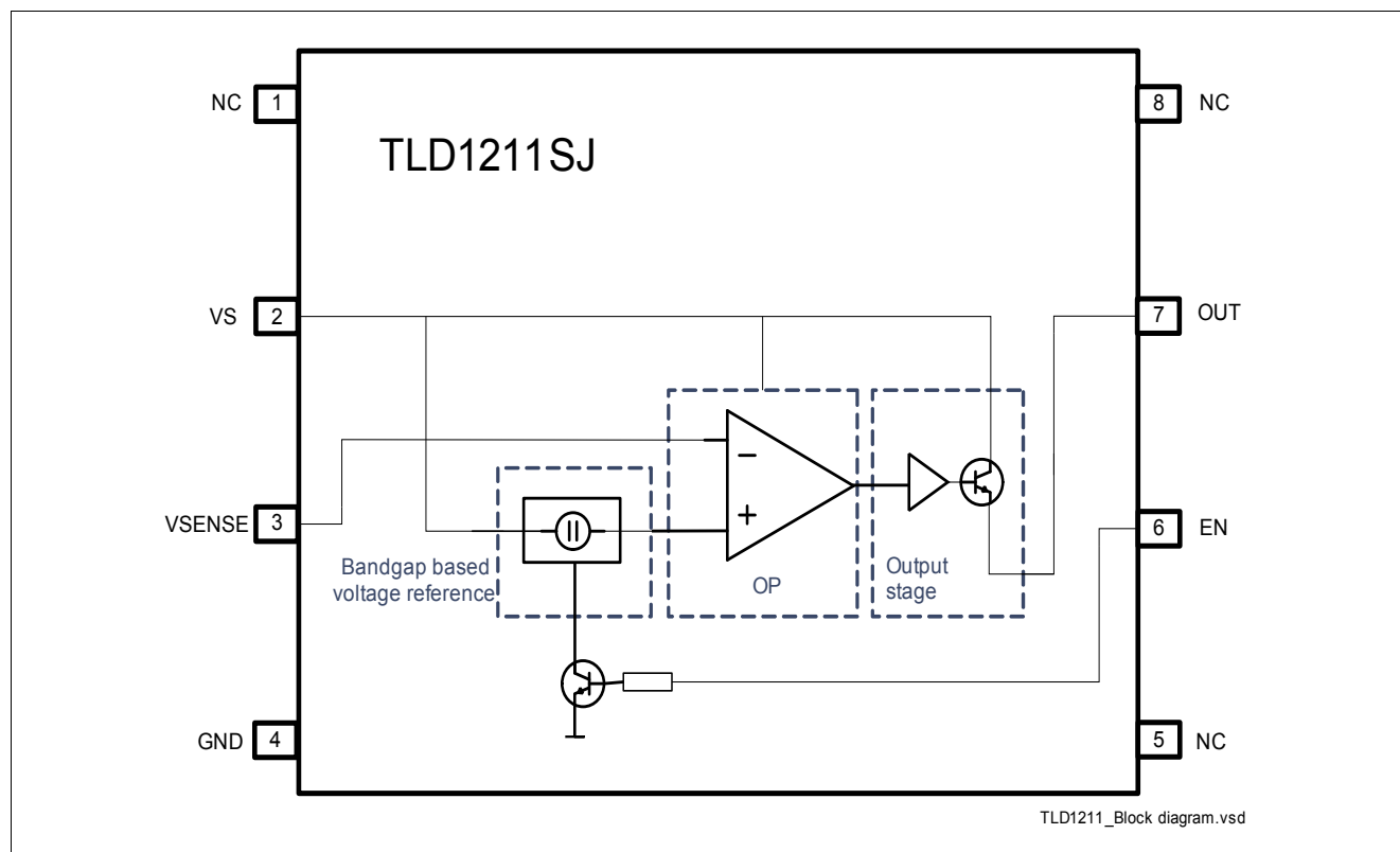
Figure 1 Block Diagram
