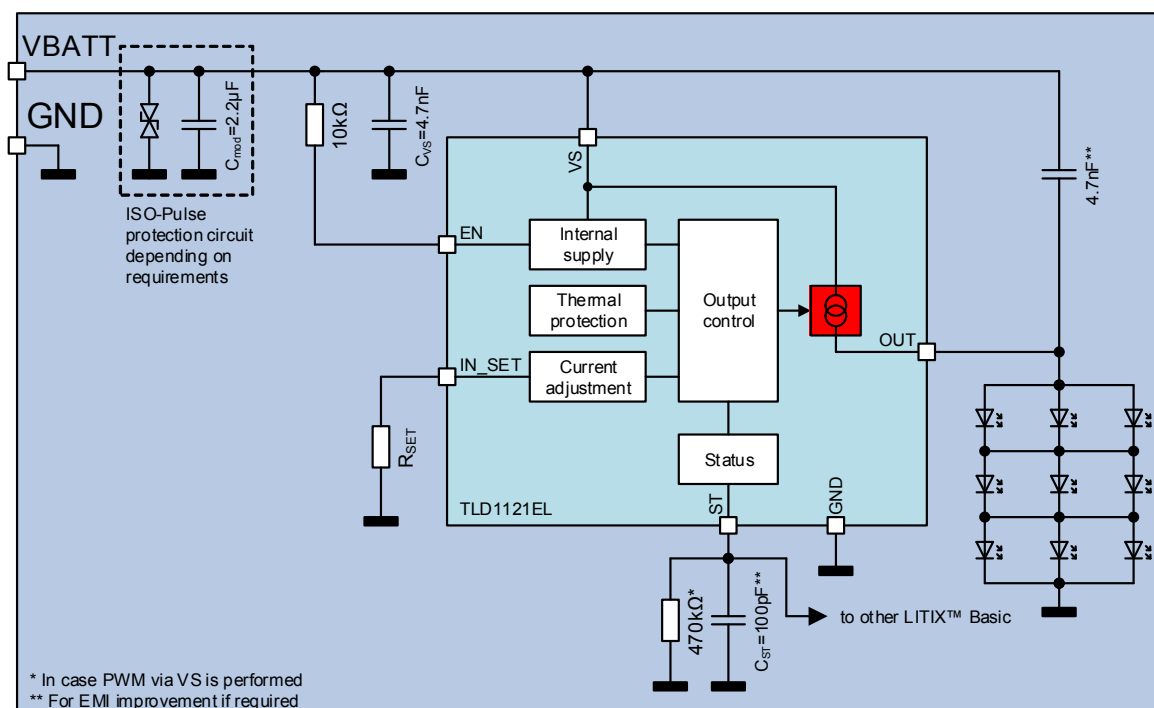
Application Diagram with TLD1121EL
