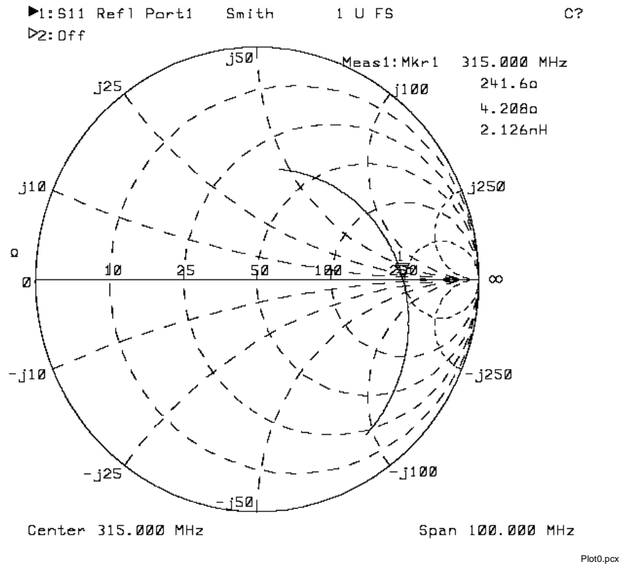
Figure 4-9 Sparam_measured_200M
