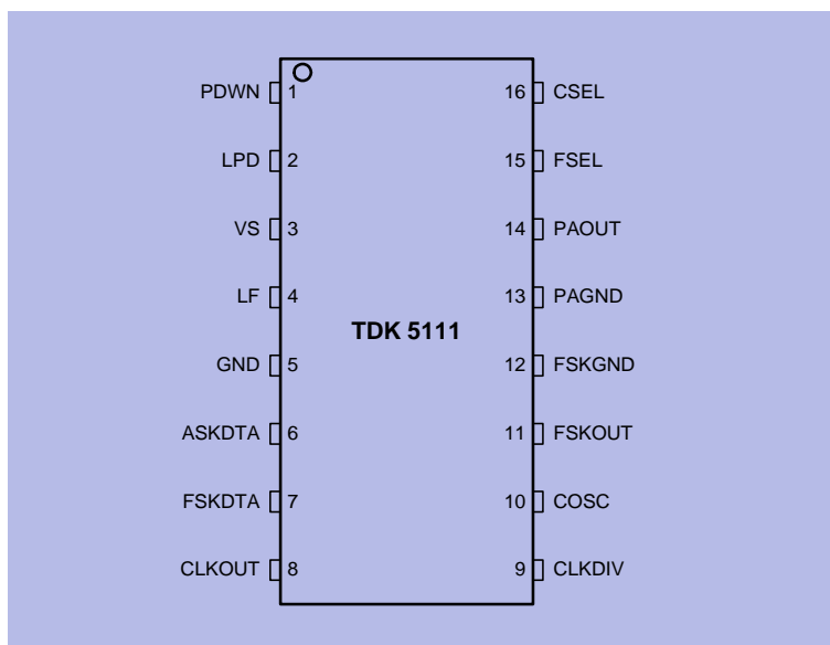
Figure 3-1 IC Pin Configuration
