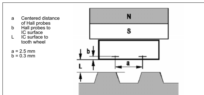
Figure 4-2 Sensor Spacing
