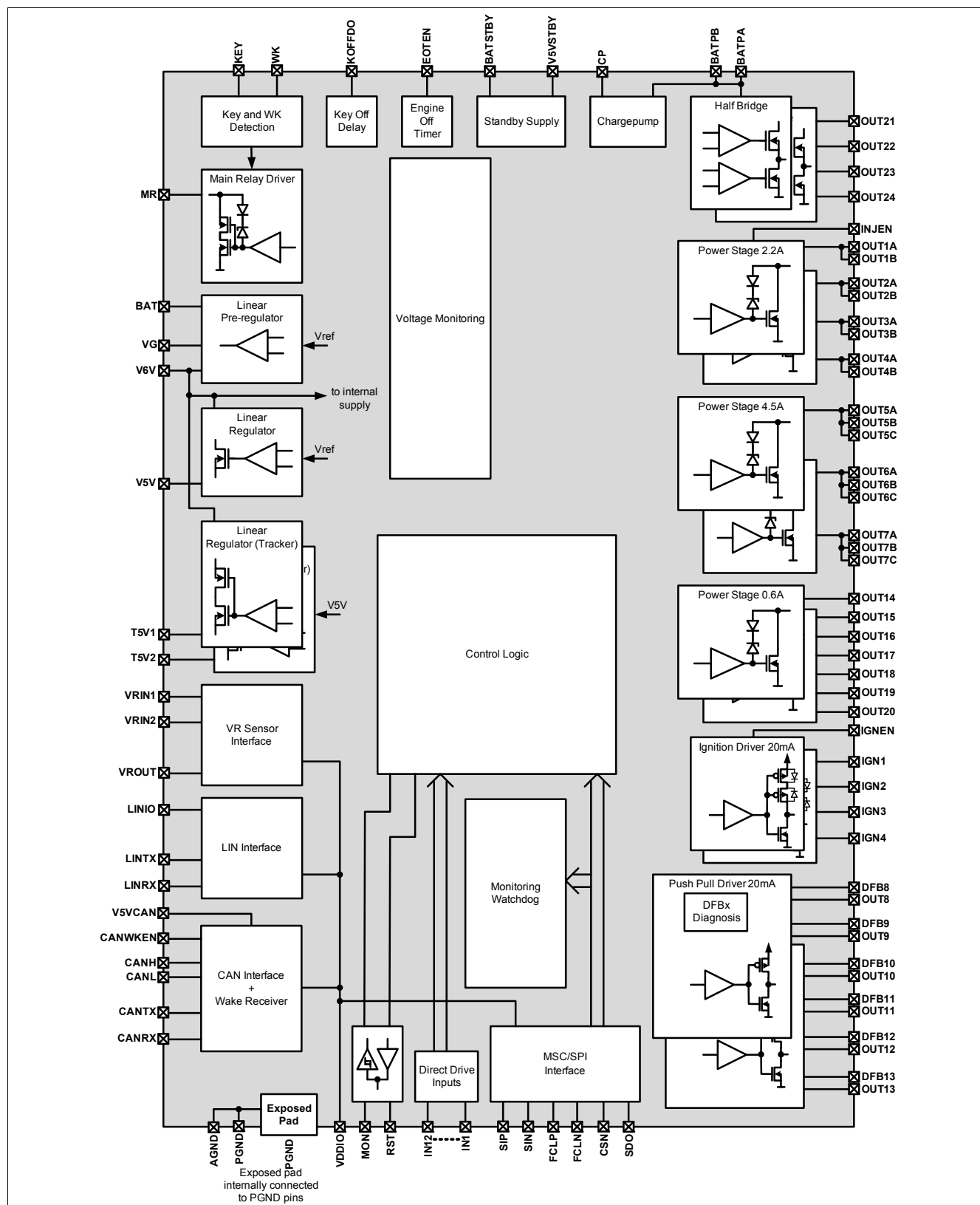
Figure 1 Block Diagram
