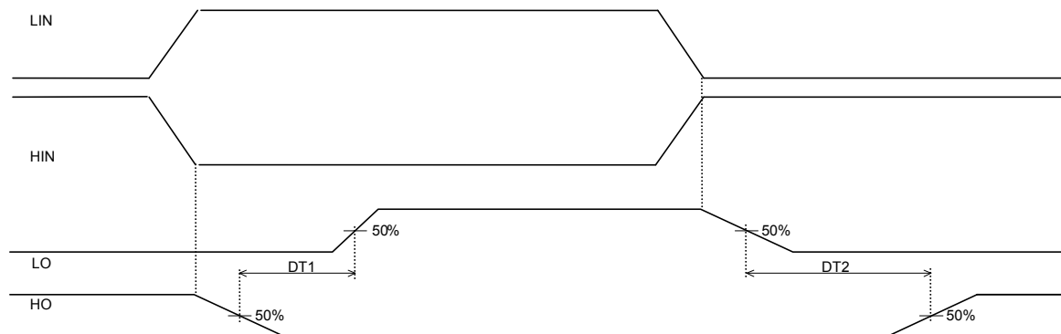
Figure 5: Deadtime definition
