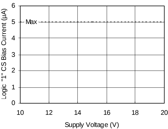
Figure 23B. Logic "1" CS Bias Current vs. Voltage
