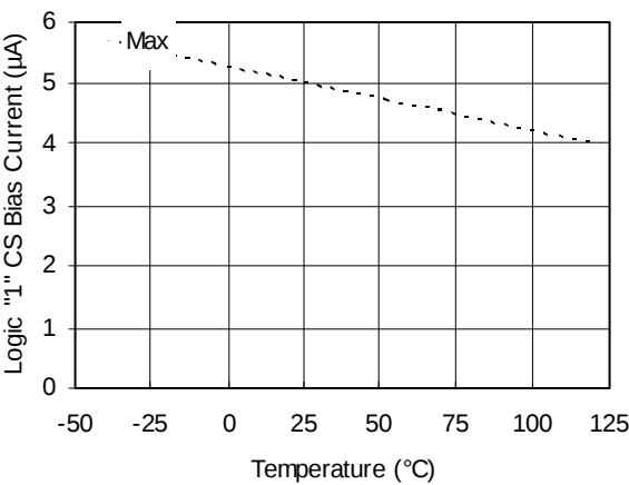
Figure 23A. Logic "1" CS Bias Current vs. Temperature
