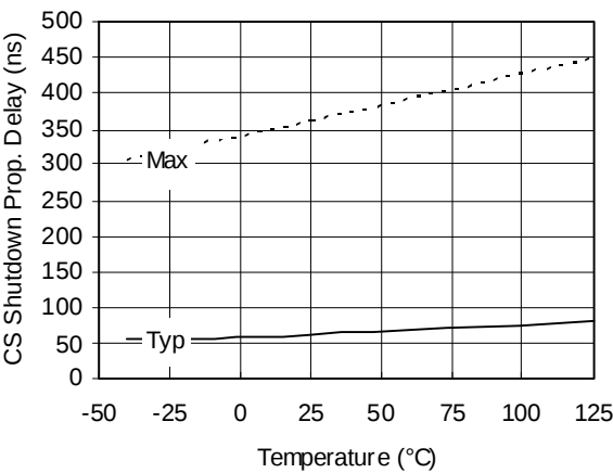
Figure 11A. CS Shutdown Prop. Delay vs. Temperature
