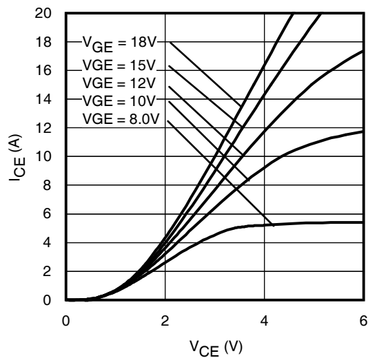
Fig. 7 - Typ. IGBT Output Characteristics T j = 150°C; tp = 80µs
