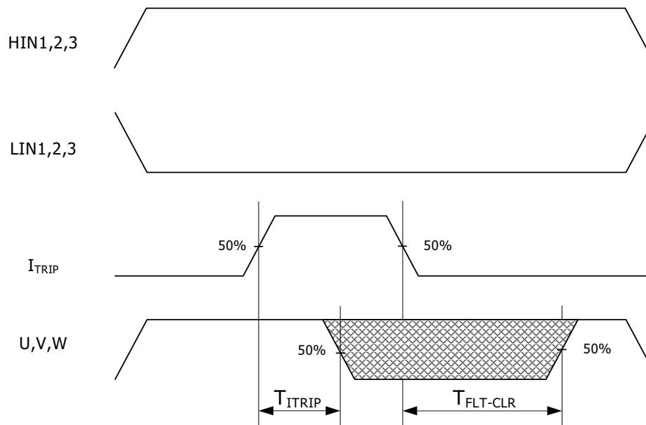
Figure 2. I_{TRIP} Timing Waveform
