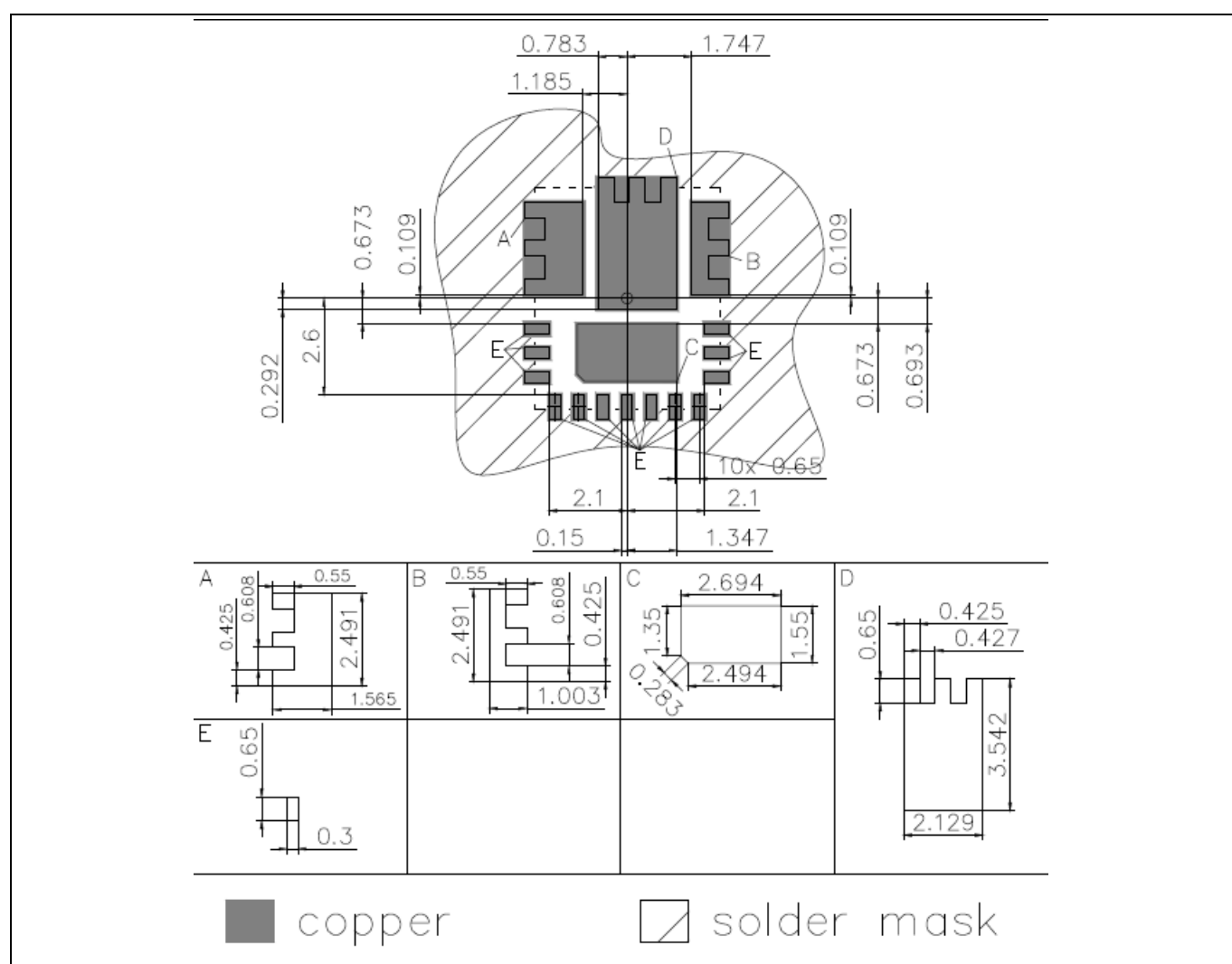
Figure 35 Solder resist
