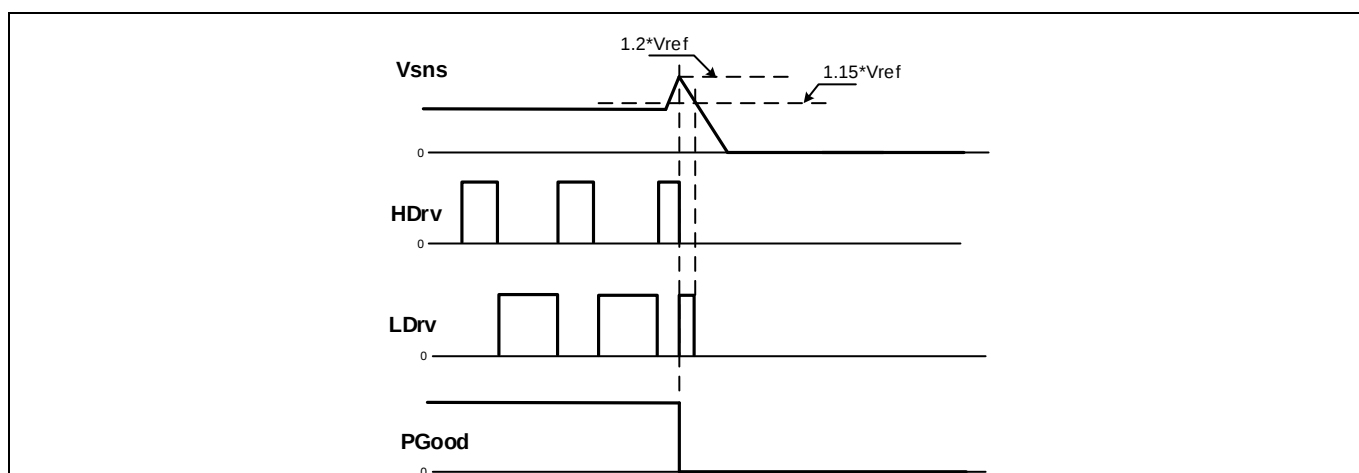
Figure 19 Timing diagram for OVP
