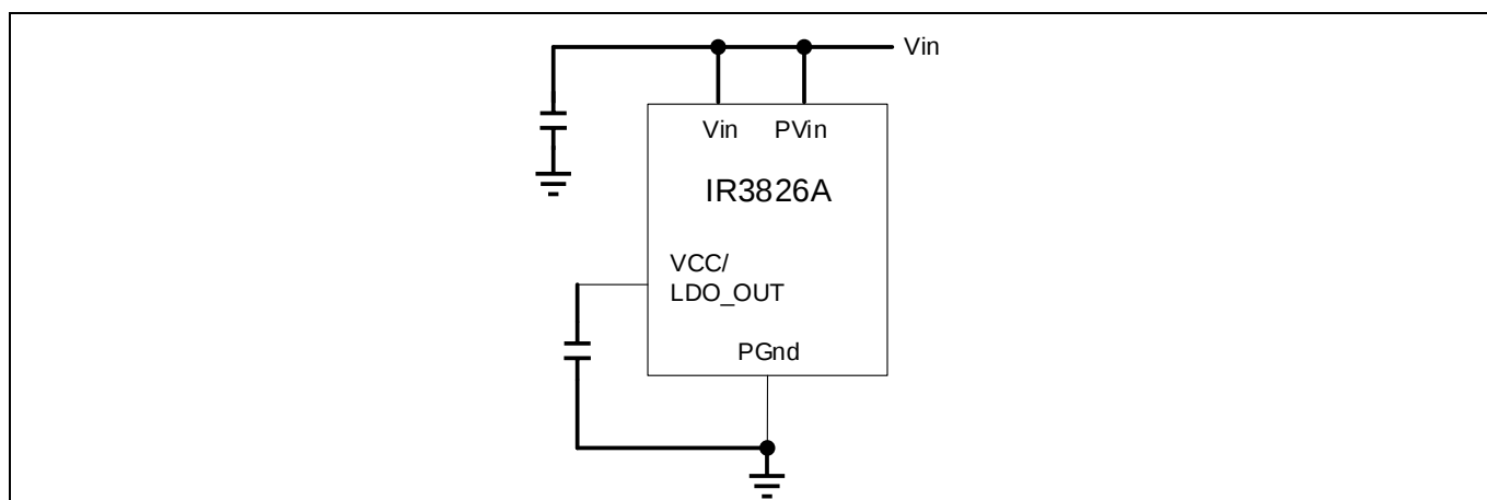
Figure 16 Internally biased single rail operation
