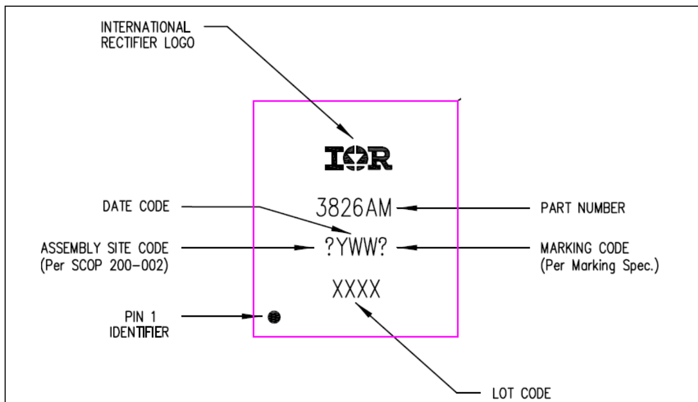
Figure 37 Package Marking
