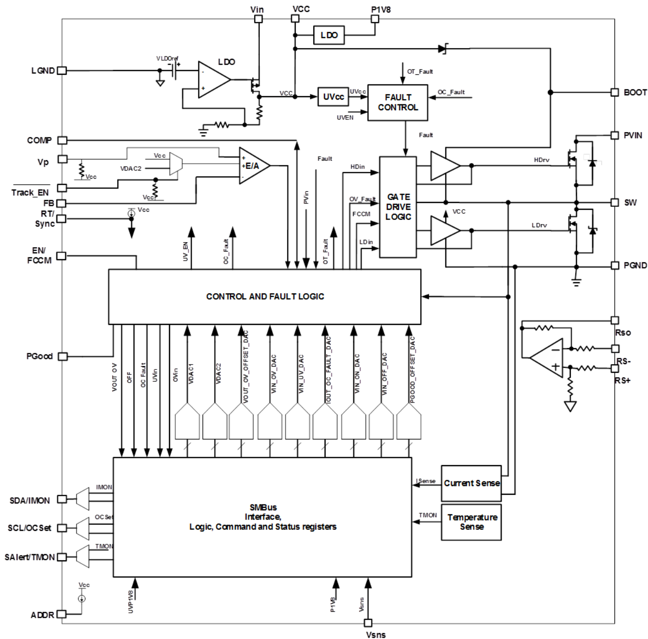
Figure 4: IR38063 Simplified Block Diagram
