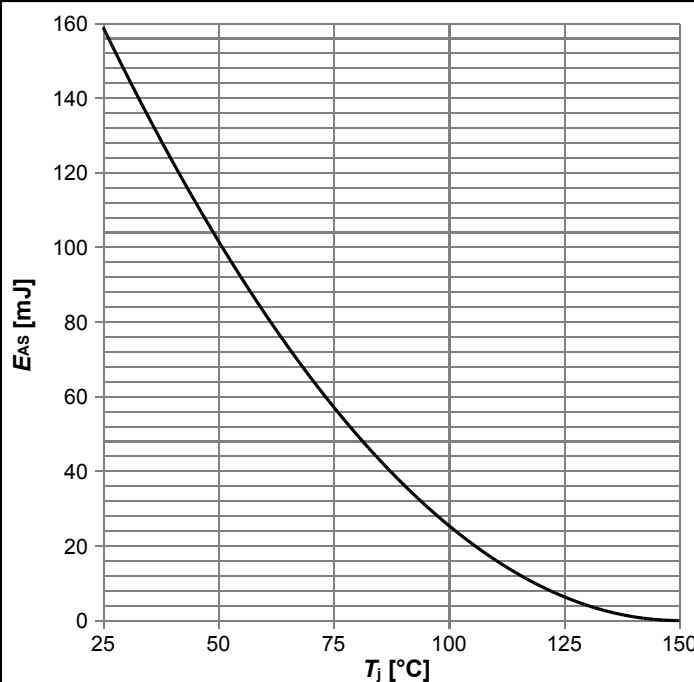
Diagram 12: Avalanche energy
