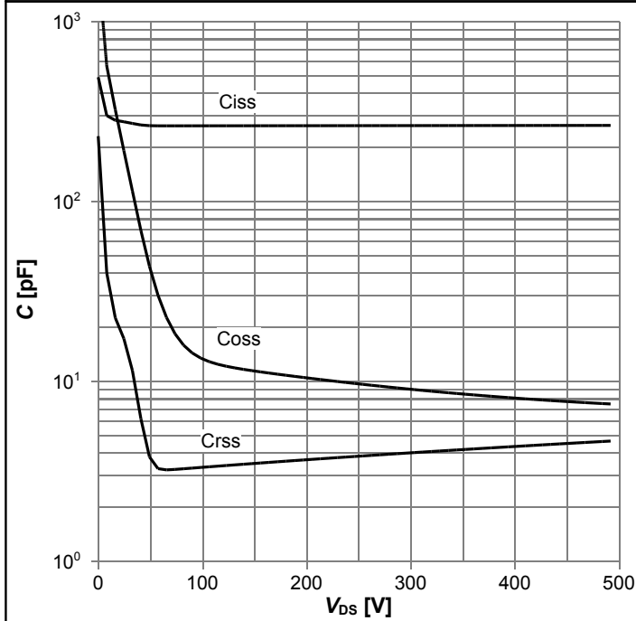
Diagram 13: Typ. capacitances
