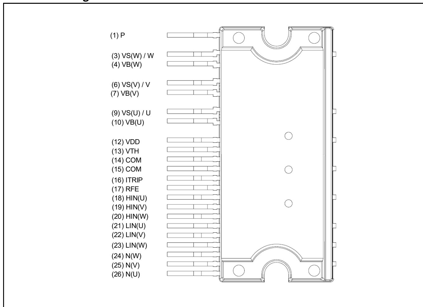
Figure 2 Pin configuration
