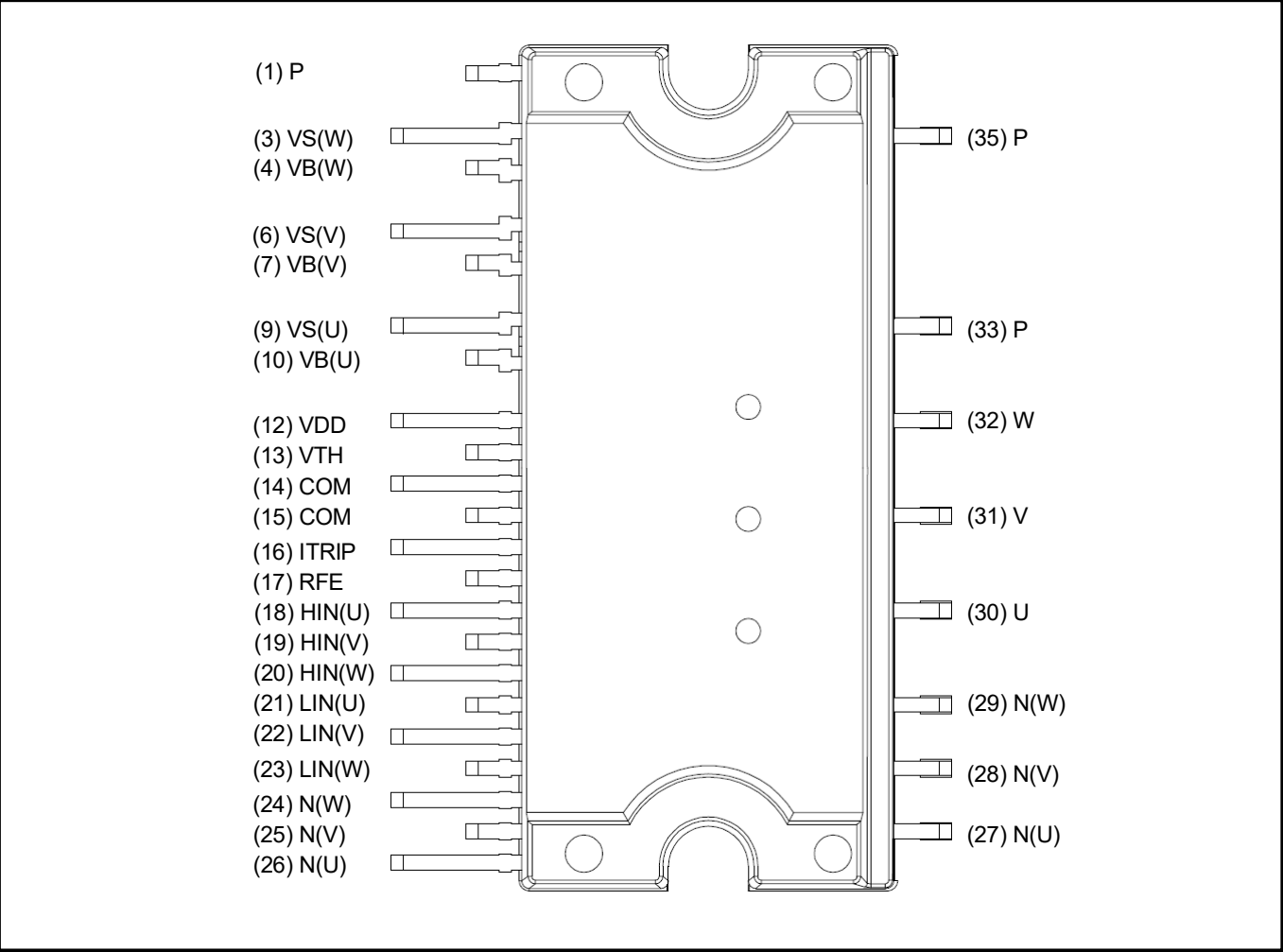
Figure 2 Pin configuration
