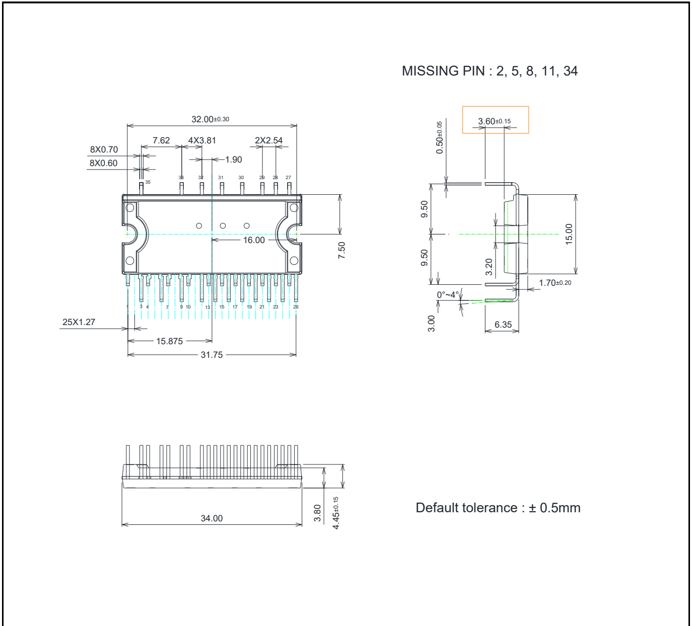
Figure 20 IM393-M6E3
