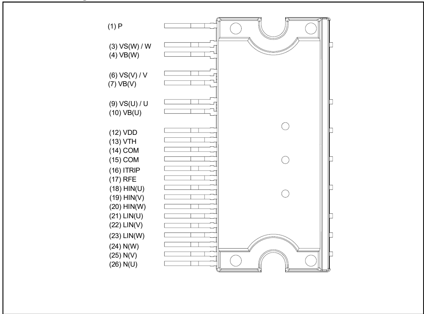
Figure 2 Pin configuration
