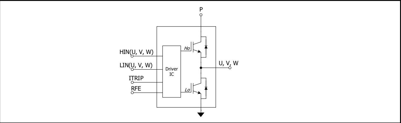
Figure 10 Module block diagram
