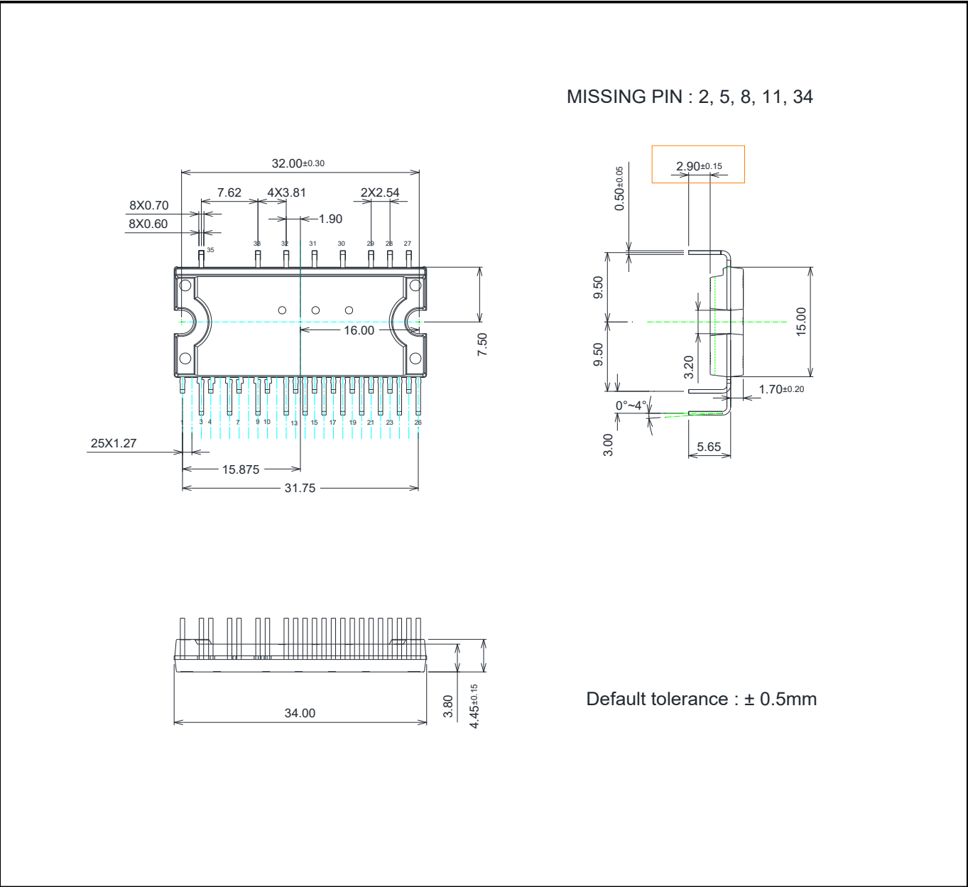
Figure 19 IM393-L6E2
