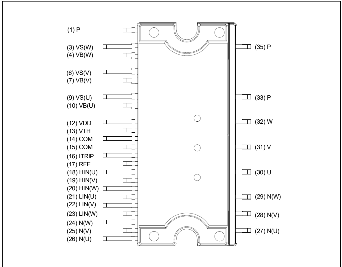
Figure 2 Pin configuration
