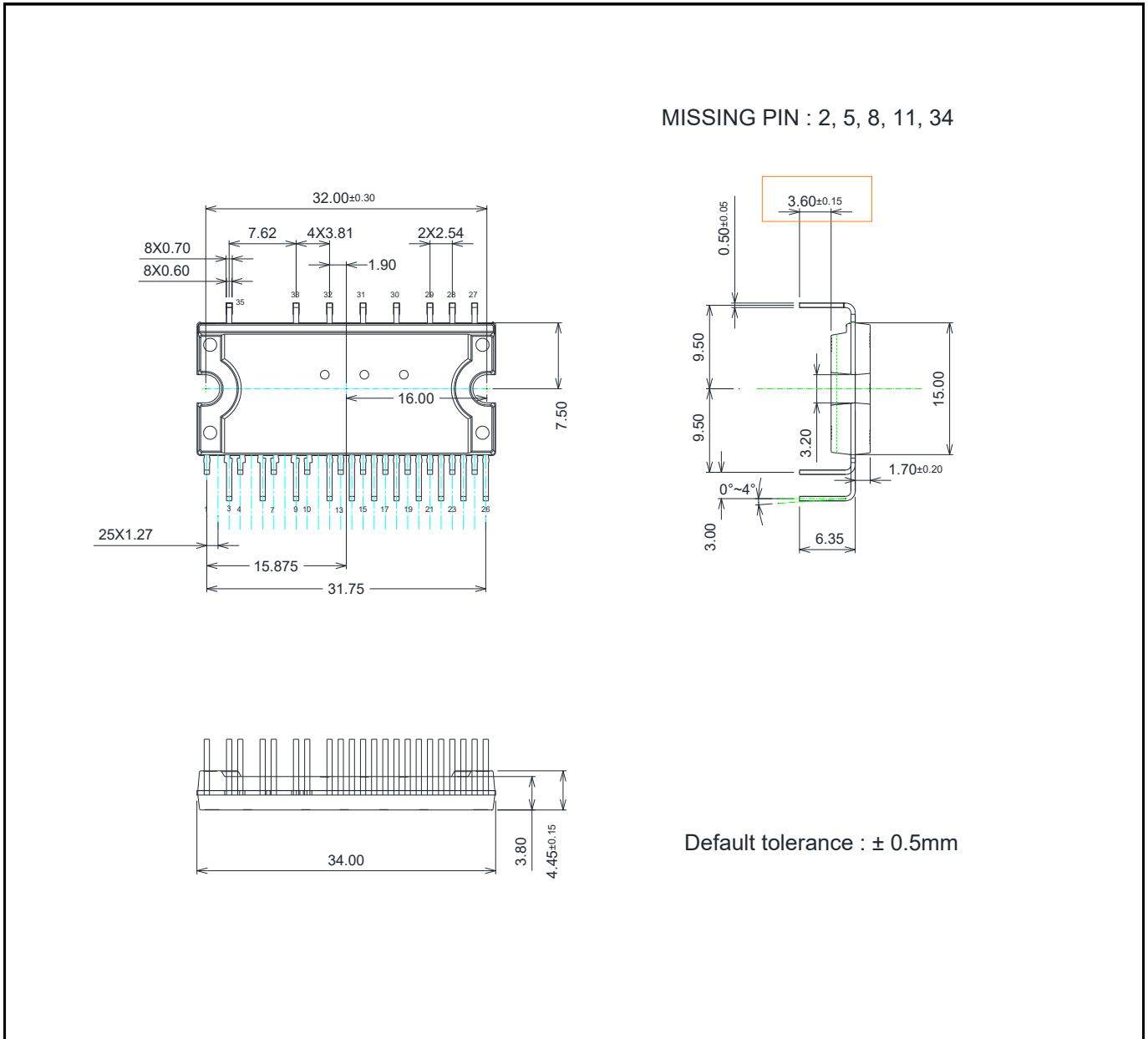
Figure 20 IM393-L6E3
