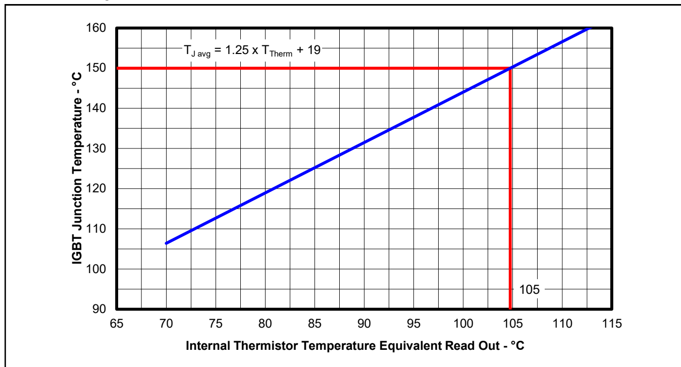
Figure 16 Typical Tj vs Tth correlation, sinusoidal modulation, V_{DC}=300\text{V} , I_{phase}=5\text{Arms} , f_{sw}=16\text{kHz} , f_{mod}=50\text{Hz} , MI=0.8 , PF=0.6
