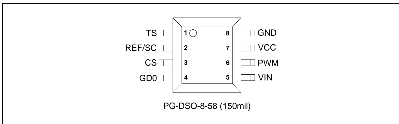
Figure 2. Pin Configuration
