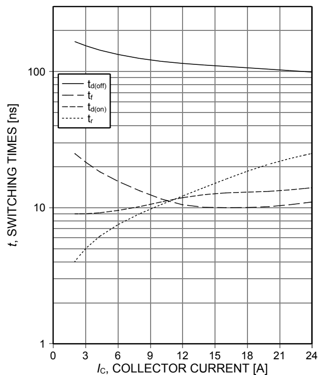
Figure 8. Typical switching times as a function of collector current (inductive load, T_j=150^\circ\text{C} , V_{CE}=400\text{V} , V_{GE}=15/0\text{V} , r_G=48\Omega , Dynamic test circuit in Figure E)
