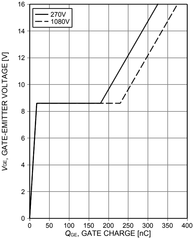
Figure 17. Typical gate charge ( I_C=40A )
