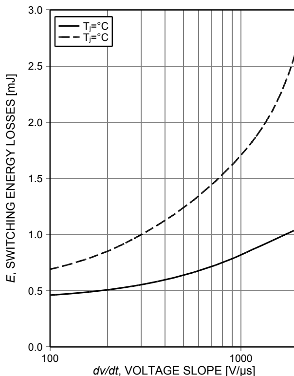
Figure 16. Typical turn off switching energy loss for soft switching (inductive load, T_{vj}=175^\circ\text{C} , V_{GE}=0/15\text{V} , I_C=40\text{A} , R_G=7.5\Omega , dynamic test circuit in Figure E)
