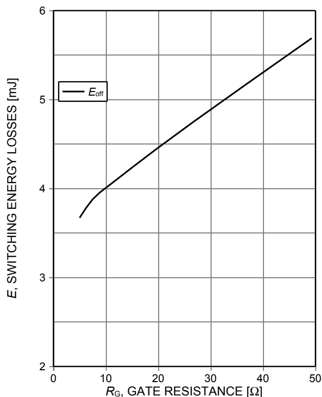
Figure 13. Typical switching energy losses as a function of gate resistance (inductive load, T_{vj}=175^\circ\text{C} , V_{CE}=600\text{V} , V_{GE}=0/15\text{V} , I_C=40\text{A} , dynamic test circuit in Figure E)
