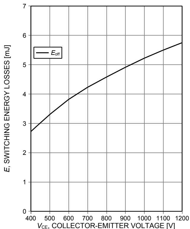
Figure 15. Typical switching energy losses as a function of collector emitter voltage (inductive load, T_{vj}=175^\circ\text{C} , V_{GE}=0/15\text{V} , I_C=40\text{A} , R_{G(on)}=7.5\Omega , R_{G(off)}=7.5\Omega , dynamic test circuit in Figure E)
