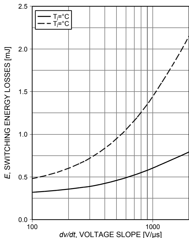
Figure 16. Typical turn off switching energy loss for soft switching (inductive load, T_{vj}=175^\circ\text{C} , V_{GE}=0/15\text{V} , I_C=30\text{A} , R_G=10\Omega , dynamic test circuit in Figure E)
