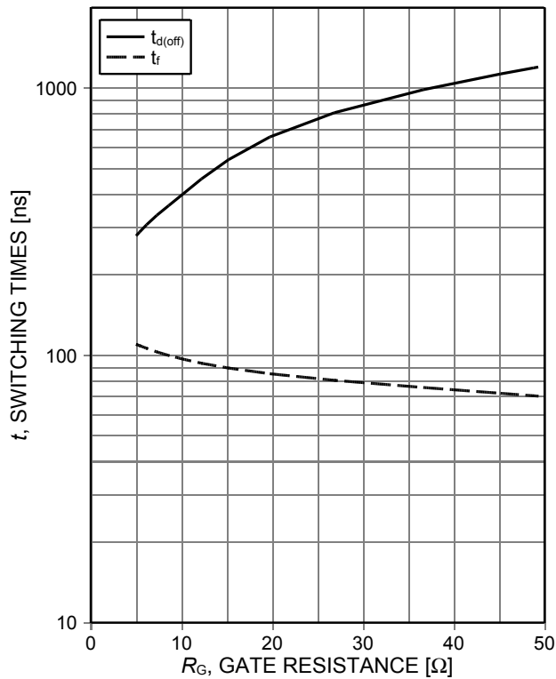
Figure 9. Typical switching times as a function of gate resistance (inductive load, T_{vj}=175^\circ\text{C} , V_{CE}=600\text{V} , V_{GE}=0/15\text{V} , I_C=30\text{A} , dynamic test circuit in Figure E)
