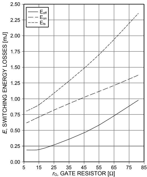
Figure 13. Typical switching energy losses as a function of gate resistor (inductive load, T_{vj}=150^\circ\text{C} , V_{CE}=400\text{V} , V_{GE}=15/0\text{V} , I_C=25\text{A} , Dynamic test circuit in Figure E)
