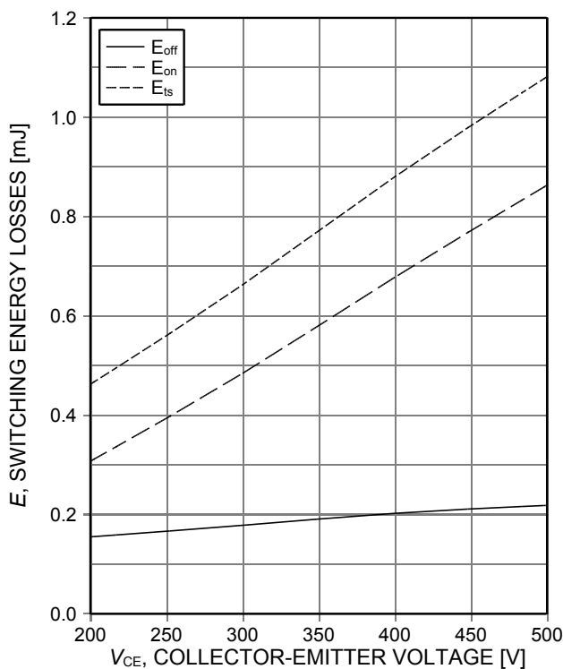
Figure 15. Typical switching energy losses as a function of collector emitter voltage (inductive load, T_{vj}=150^\circ\text{C} , V_{GE}=15/0\text{V} , I_C=25\text{A} , r_G=12\Omega , Dynamic test circuit in Figure E)
