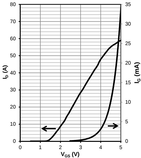
Figure 12 Typ. transfer characteristics
