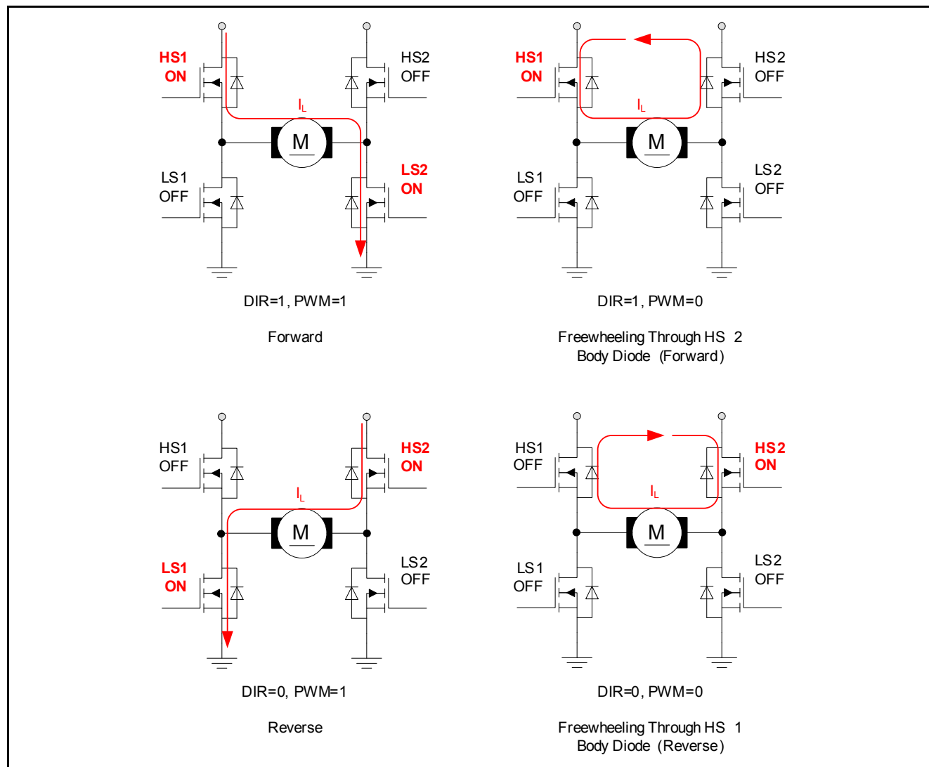
Figure 4-2 Operation Modes
