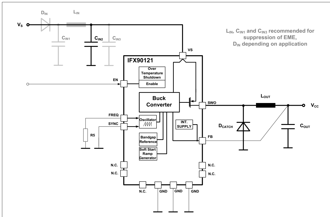
Figure 8 Application diagram
