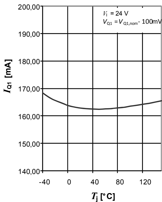
Output Current Limitation I_{Q1} versus Junction Temperature T_j (@ V_{Q1, \text{nom}} - 100\text{mV} )
