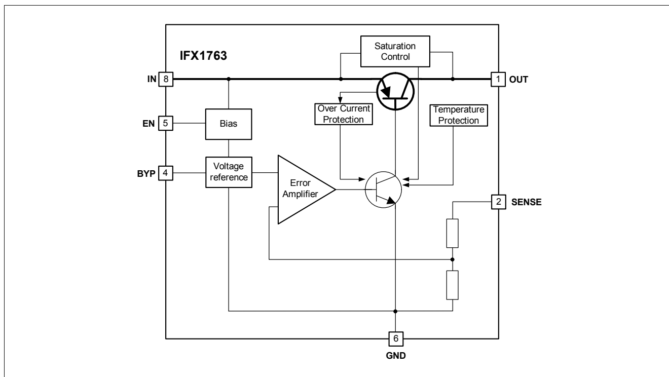
Figure 1 Block Diagram IFX1763 V50
