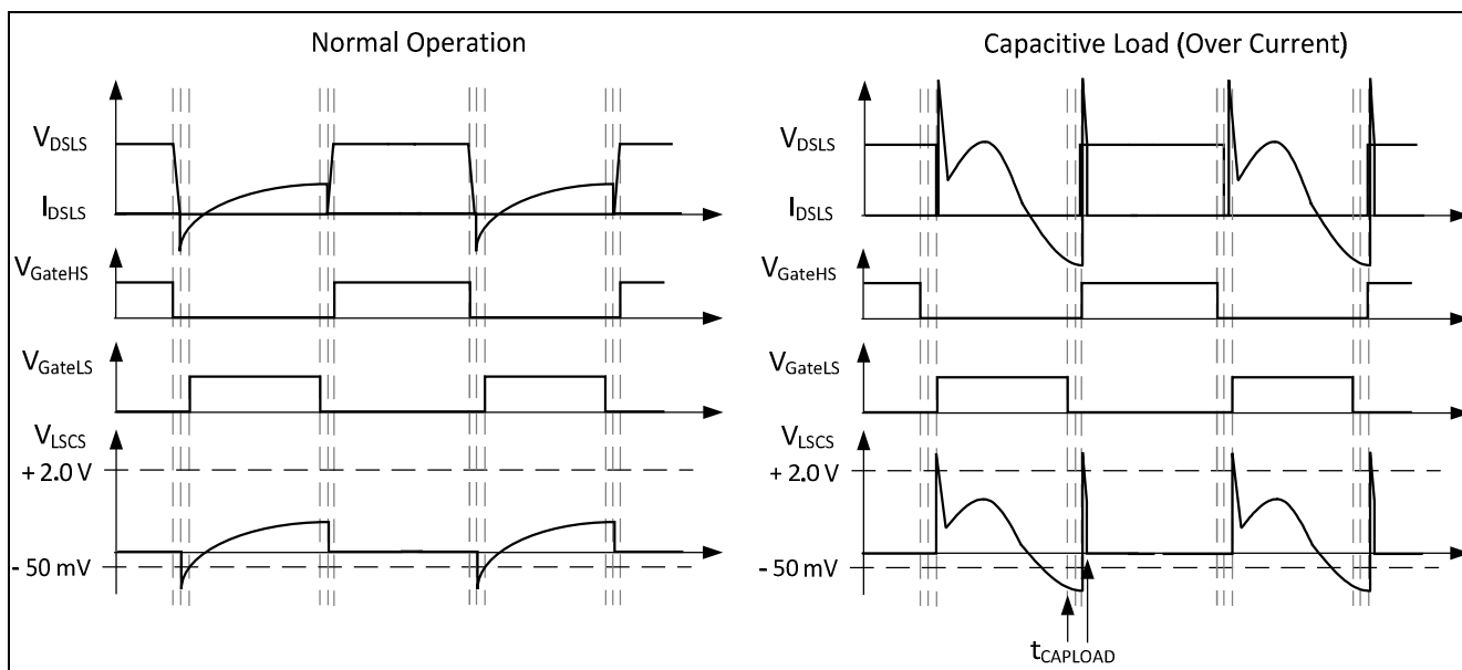
Figure 8 Capacitive Mode Operation
