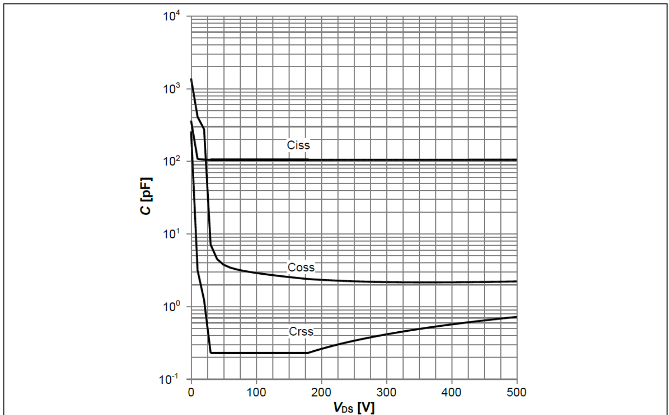
Figure 26 Typical CoolMOS™ capacitances of ICE5AR4780BZS ( C=f(V_{DS}); V_{GS}=0 V; f=250 kHz)
