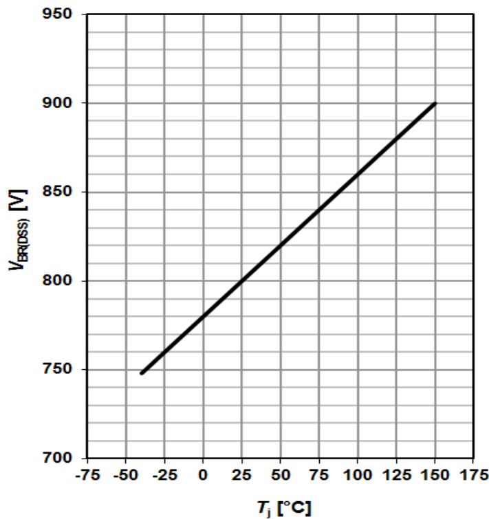
Figure 24 Drain-source breakdown voltage ICE5ARxx80BZS; V_{BR(DSS)}=f(T_J) , I_D=1 mA
