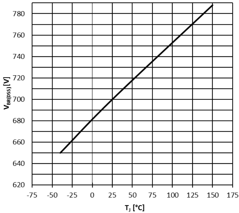
Figure 23 Drain-source breakdown voltage ICE5ARxx70BZS; V_{BR(DSS)}=f(T_J) , I_D=1 mA
