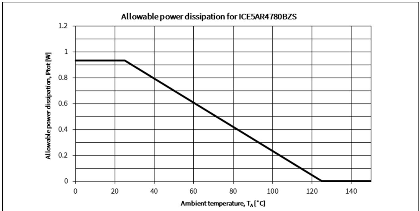
Figure 21 Power dissipation of ICE5AR4780BZS; P_{\text{tot}}=f(T_a) , (Maximum ratings as given in section 4.1 must not be exceeded)
