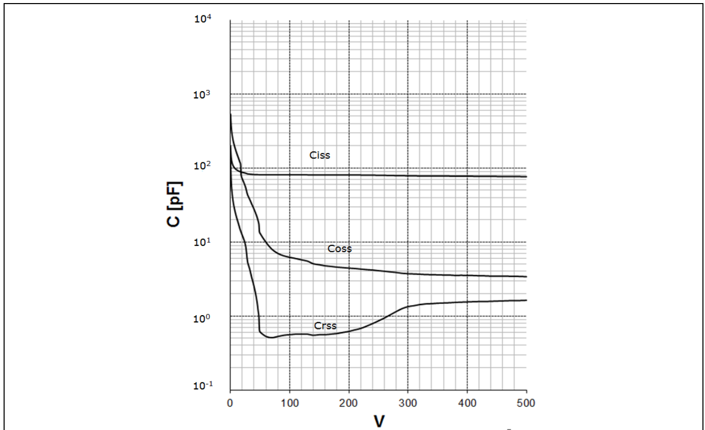
Figure 25 Typical CoolMOS™ capacitances of ICE5AR4770BZS ( C=f(V_{DS}); V_{GS}=0 V; f=1 MHz)
