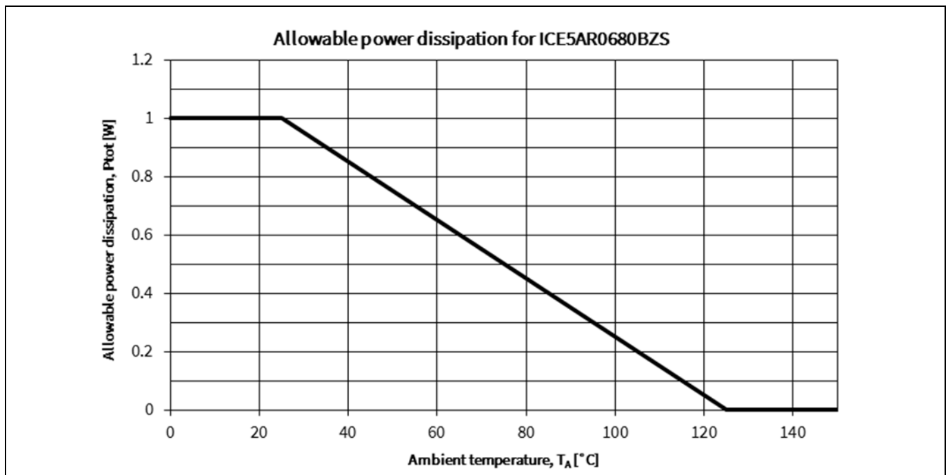
Figure 22 Power dissipation of ICE5AR0680BZS; P_{\text{tot}}=f(T_a) , (Maximum ratings as given in section 4.1 must not be exceeded)
