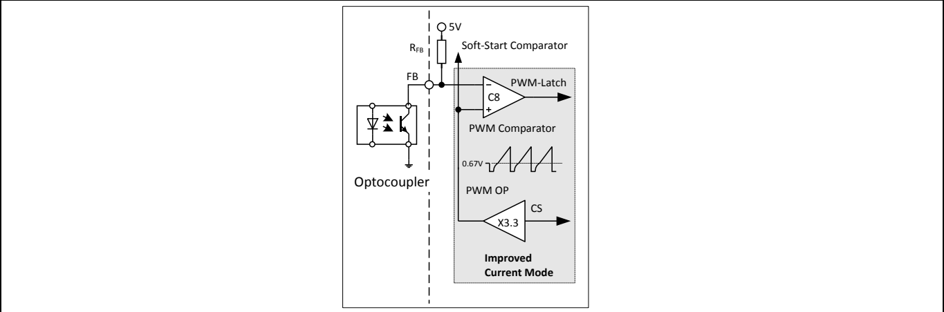
Figure 9 PWM Controlling
