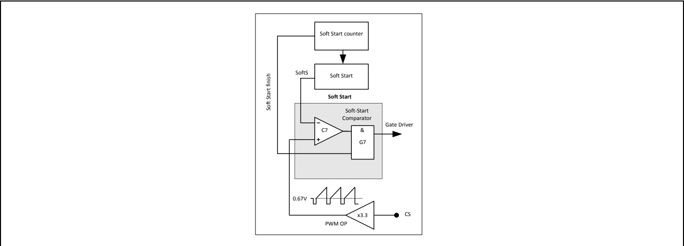
Figure 10 Soft Start
