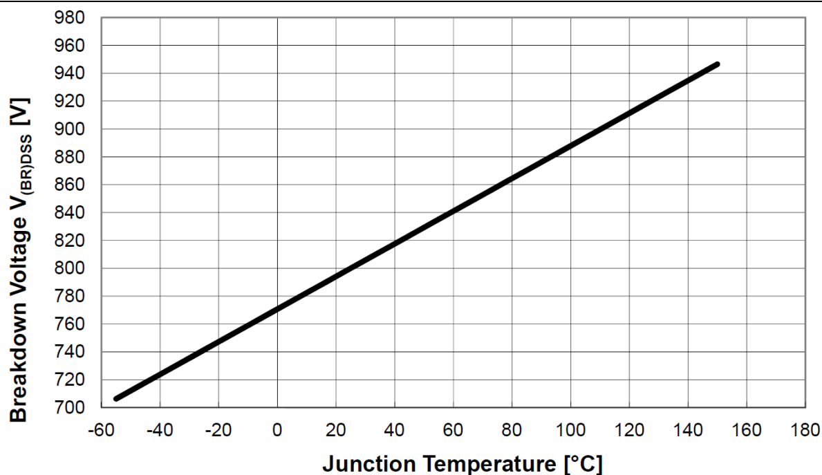
Figure 39 Drain-source breakdown voltage; V_{BR(DSS)}=f(T_j) , I_D=0.25\text{mA}
