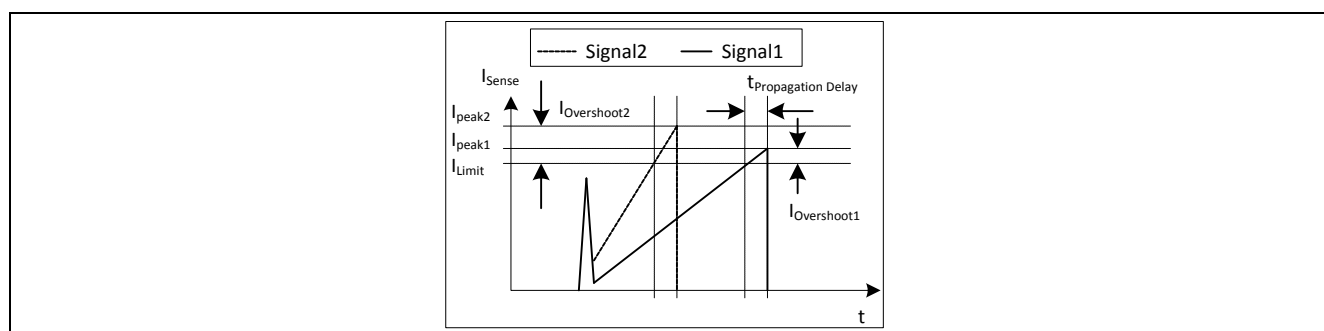
Figure 20: Current Limiting
