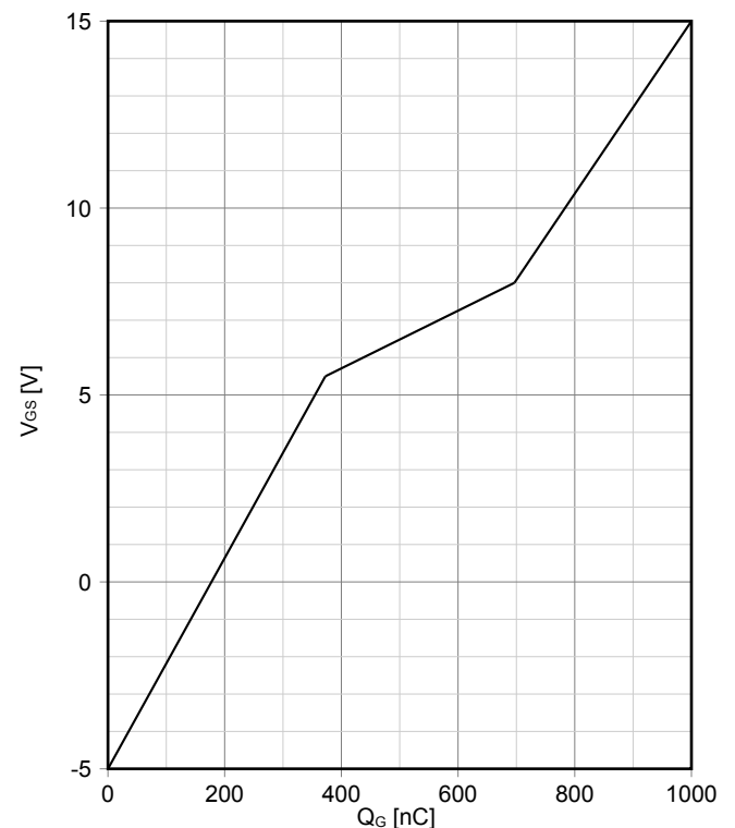
Gateladungs Charakteristik MOSFET (typisch) gate charge characteristic MOSFET (typical)
