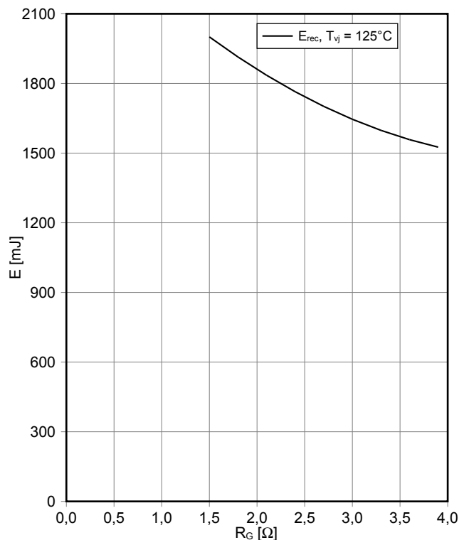
开关损耗 二極體, 反轉 (典型) switching losses Diode, Reverse (typical) E_{rec} = f(R_G) I_F = 500 \text{ A} , V_{CE} = 3600 \text{ V}
