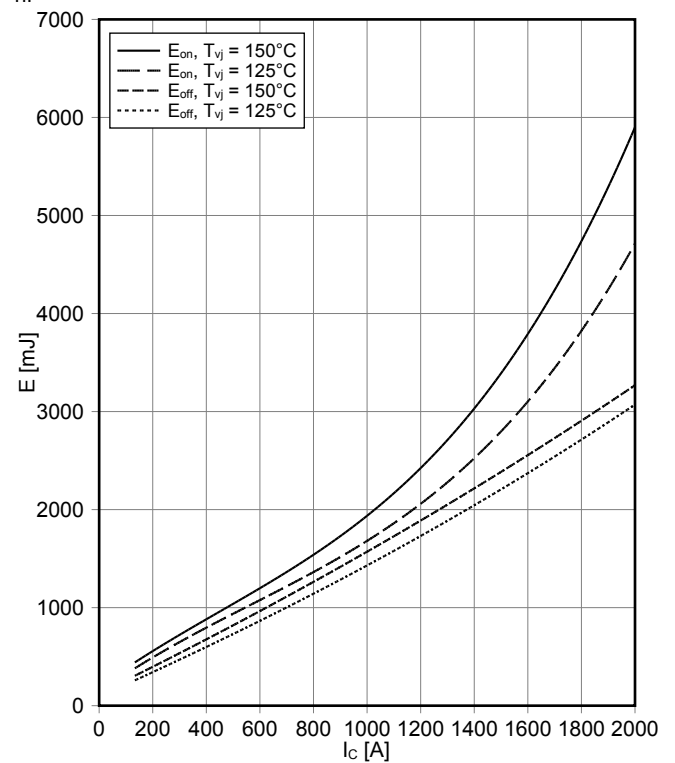
开关损耗 IGBT, 制动-斩波器 (典型) switching losses IGBT, Brake-Chopper (typical) E_{on} = f(I_C) , E_{off} = f(I_C) V_{GE} = \pm 15\text{ V} , R_{Gon} = 0.71\ \Omega , R_{Goff} = 2.3\ \Omega , V_{CE} = 1800\text{ V} , C_{GE} = 220\text{ nF}
