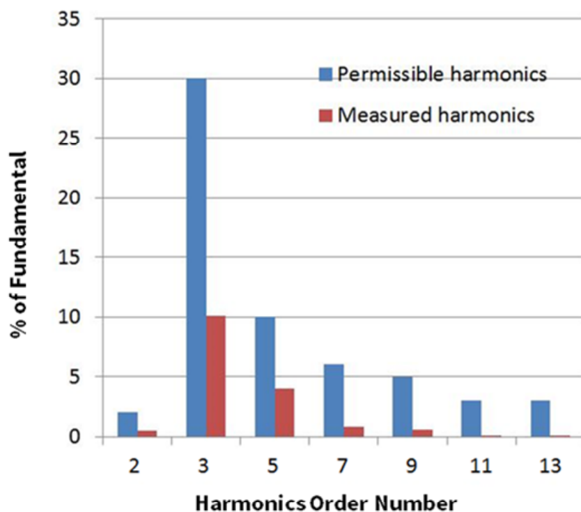
Figure 9 Line current harmonics V AC = 90 V/60 Hz, 30 percent dimming
