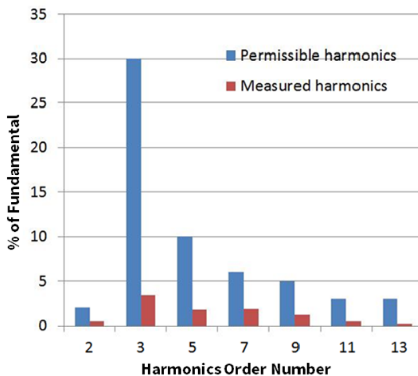
Figure 10 Line current harmonics V AC = 230 V/50 Hz, 100 percent dimming
