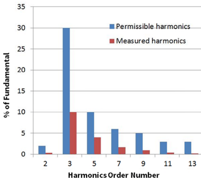
Figure 13 Line current harmonics V AC = 277 V/60 Hz, 30 percent dimming
