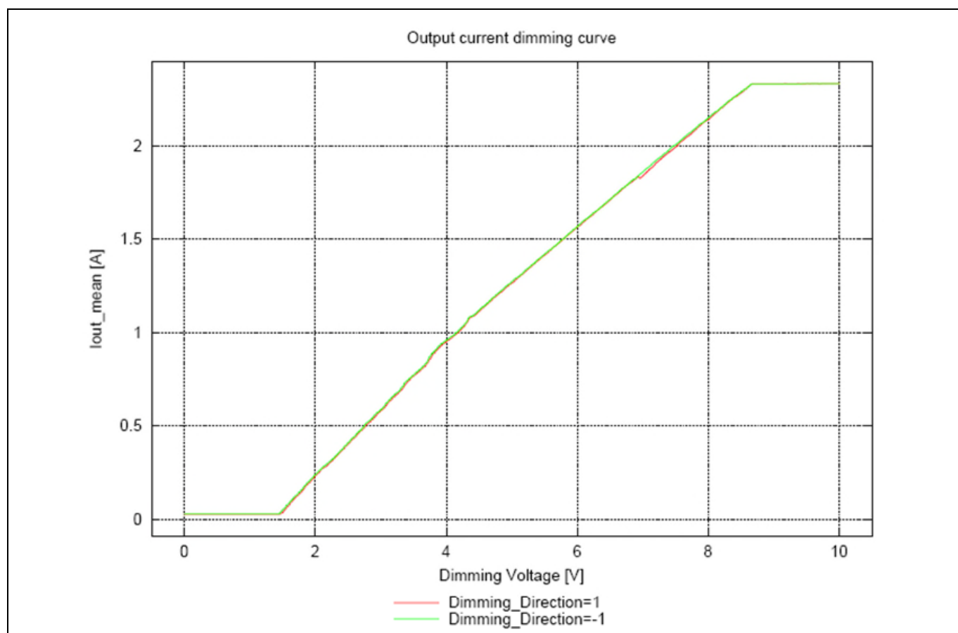
Figure 14 XDPL8221 100 W reference board linear dimming curve with V AC = 230 V/50 Hz, 13 LEDs
