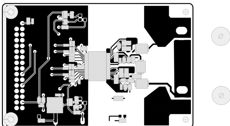
Figure 4-6 Layout top of the EVAL_2ED020I12-F2
