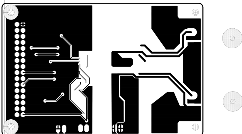
Figure 4-7 Layout bottom of the EVAL_2ED020I12-F2
