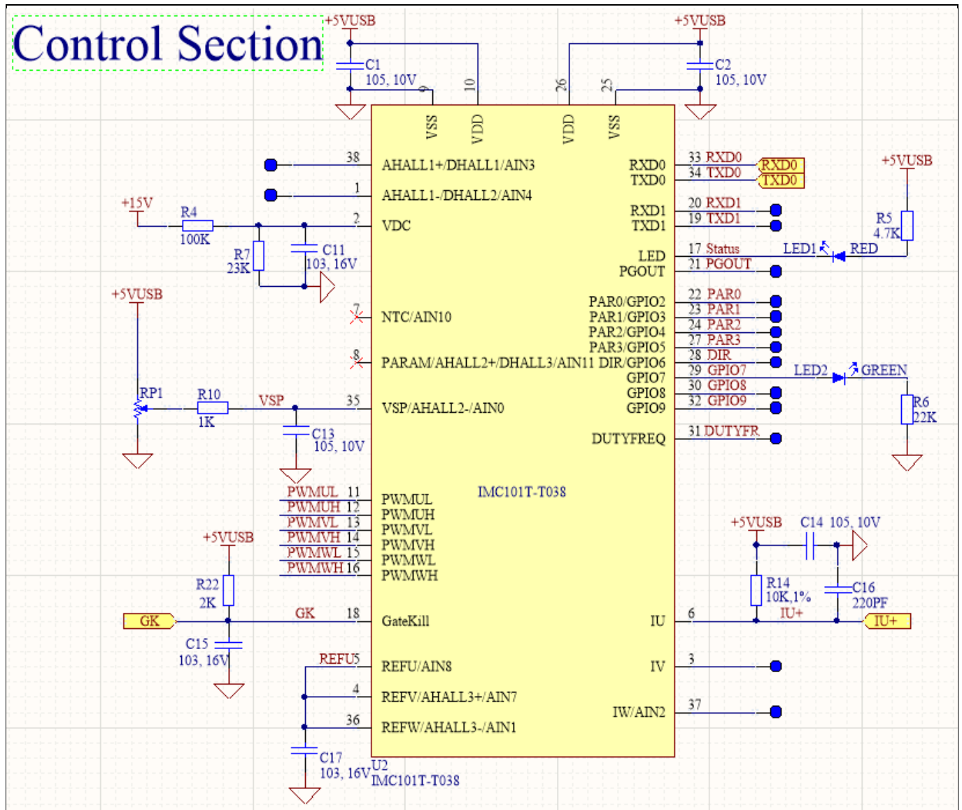
Figure 5 Controller
