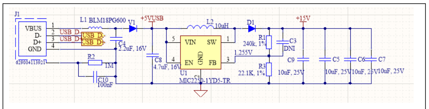
Figure 6 Power supplies
