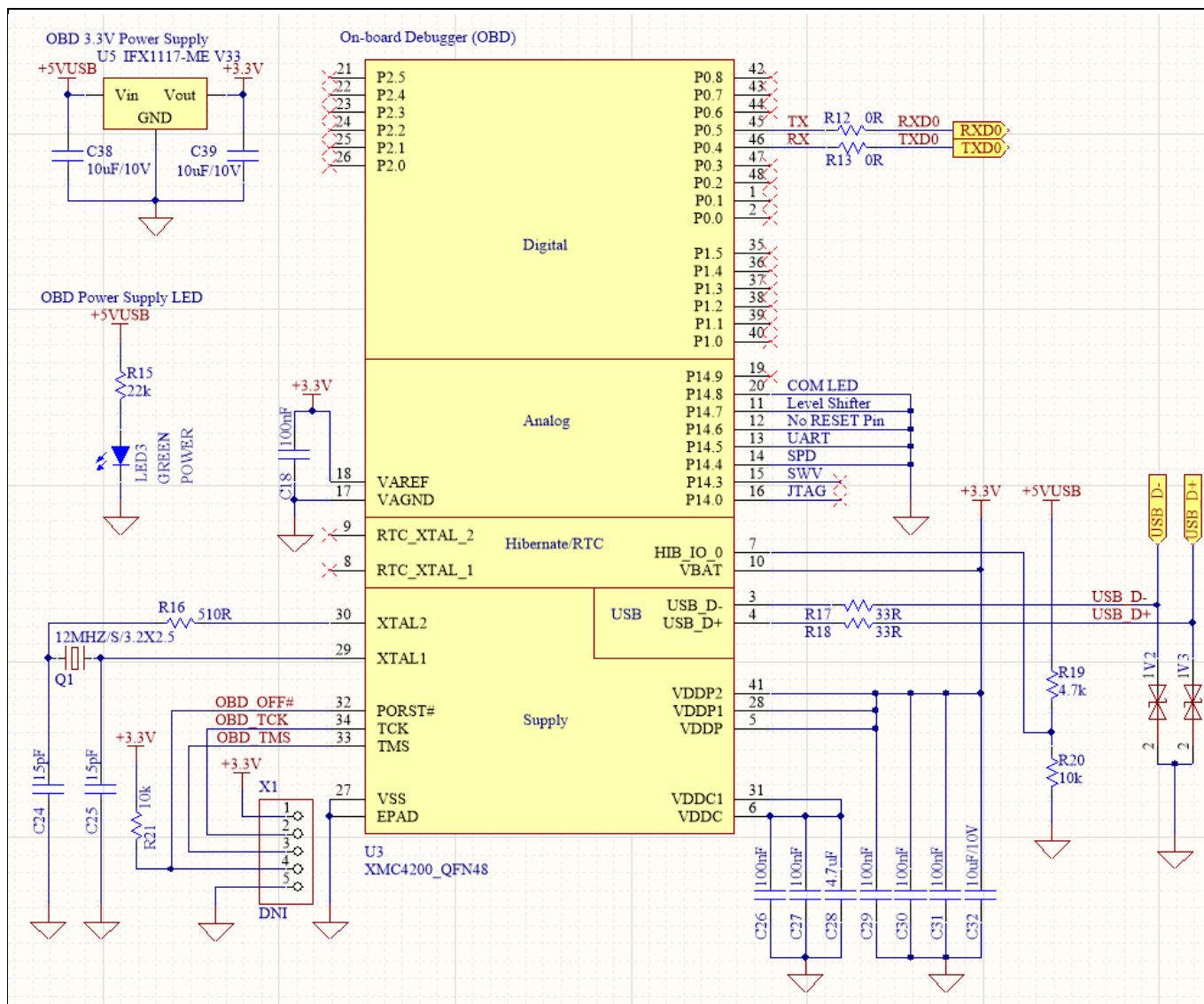
Figure 4 On-board debugger
