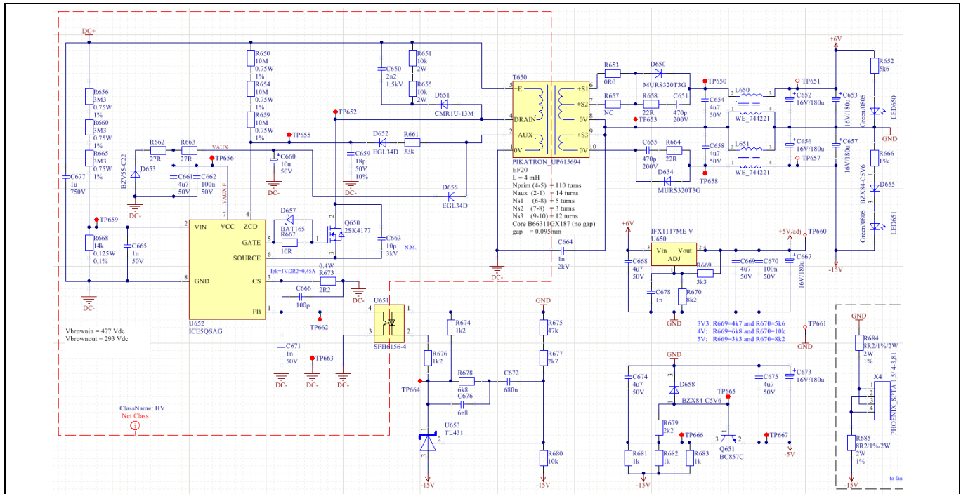
Figure 8 Auxiliary supply
