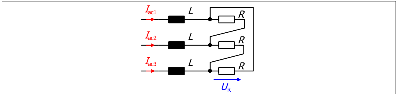
Figure 23 Test load
